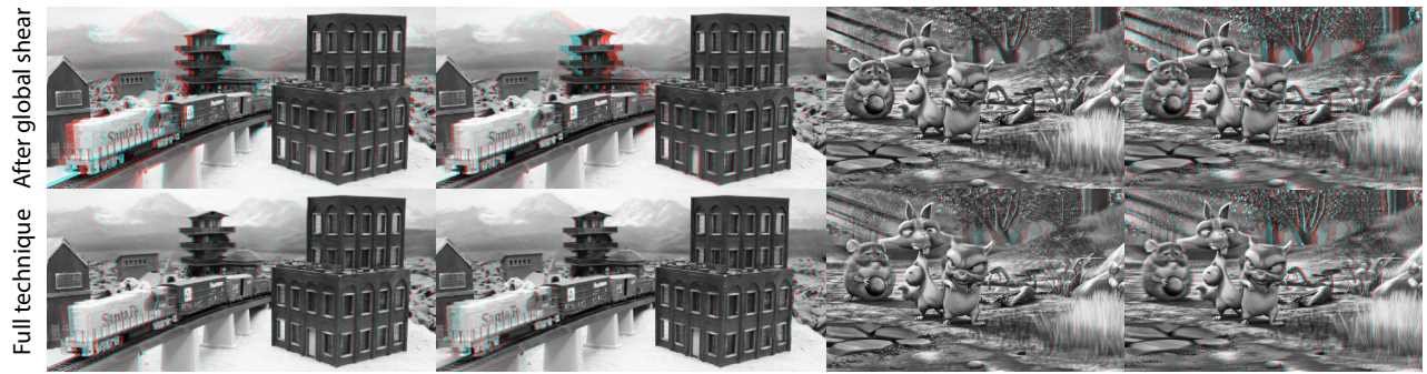
Figure 12: The comparison of the results obtained using full technique and only global shearing on an automultiscopic screen (simulation). For better perception of depth, we remove the colors and show a monochrome anaglyph; please refer to the supplementary materials for full results.
