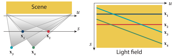
Figure 4: The figure visualizes a scene together with its light field in the two-plane parametrization. Images observed on the screen correspond to linear cuts through the epipolar-plane images. While views located on the s axis correspond to horizontal lines, viewing positions, which are away from the axis, result in slanted lines. As slants encode the distance to the scene, two viewing positions located at the same distance result in parallel lines.
