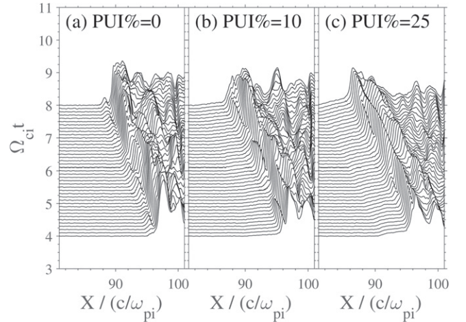
Figure 4. Stack plots of the B profiles (at Y = 0 ) at different times. From left to right, the relative density of PUIs is 0%, 10%, and 25%, respectively.
