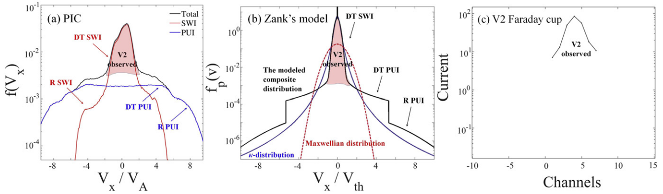
Figure 9. (a) Velocity distribution of the ions (black) selected in the “DS box” (see Figure 7) of the TS. Contributions of SWIs and PUIs to the total distribution are indicated by red and blue curves, respectively. The highlighted region (cool core) at the peak of the distribution is expected to be observed by V2. (b) Heliosheath particle distribution (black) modeled by Zank et al. (2010). The Maxwellian (red) and \kappa (blue) distributions with the same temperature and particle density are also shown for reference. (c) Cool core of the ion distribution observed by V2 in the downstream region of TS-3.
