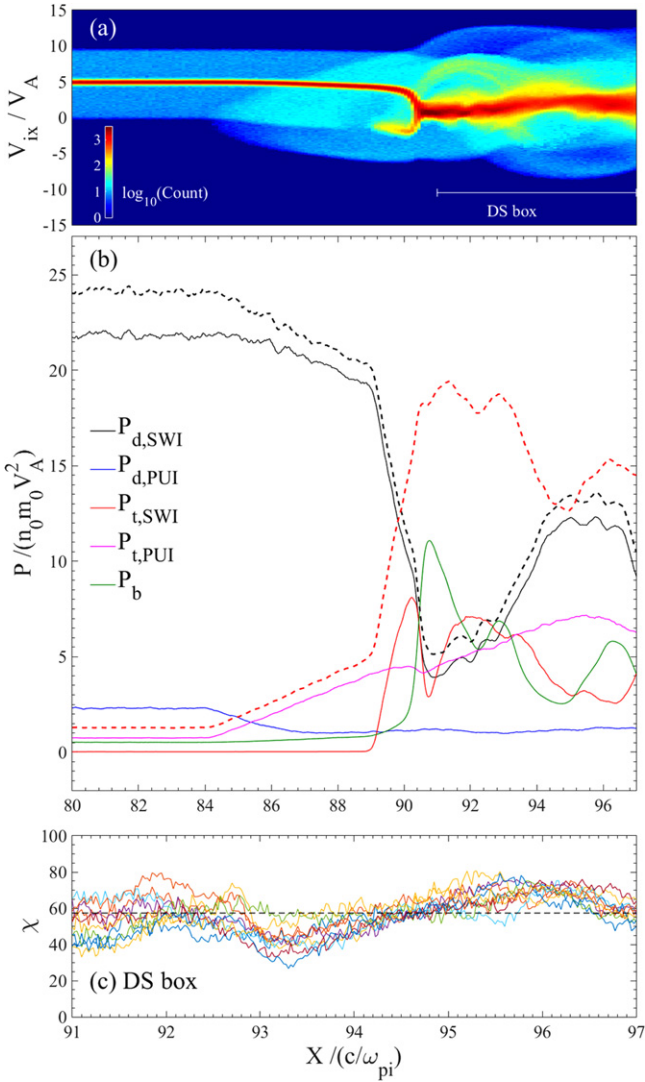
Figure 6. (a) Phase space plots of the SWIs and PUIs at t = 7 \Omega_{ci}^{-1} in Run B (PUI% = 10). The color shading shows logarithmic distributions of the particle number. (b) The dynamic pressure of SWIs (black) and PUIs (blue), the thermal pressure of SWIs (red) and PUIs (magenta), and the magnetic pressure (green) across the shock front. The black dashed curve indicates the total ion dynamic pressure. The red dashed curve indicates the sum of the total ion thermal pressure and the magnetic pressure. (c) The pressure ratio \chi = P_t^{\text{PUI}}/P_t computed in a downstream region (marked by “DS box” in the top panel).
