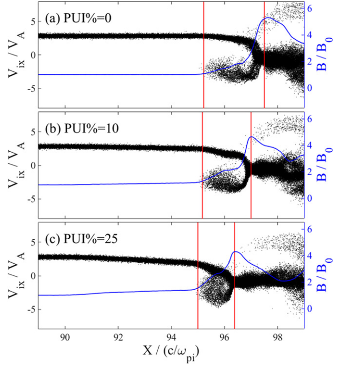
Figure 3. Phase space plots ( V_{ix} vs. X ) of SWIs at t = 4 \Omega_{ci}^{-1} . From top to bottom, the relative densities of the PUIs are 0%, 10%, and 25%, respectively. In each panel, the Y -averaged B field (blue curve) is shown for reference. The ripple region is between the two vertical red lines.
