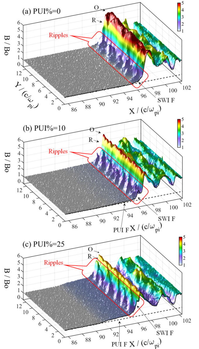
Figure 1. Overview of the magnetic field profiles at a time t = 4 \Omega_{ci}^{-1} for (a) PUI% = 0, (b) PUI% = 10, and (c) PUI% = 25. The color shading indicates the strength of the magnetic field. The shock foot, ramp, and overshoot are marked by “F,” “R,” and “O,” respectively. The foot regions due to the reflected PUIs and SWIs are labeled as “PUI F” and “SWI F,” respectively. The dashed black reference line shows the upstream value B_0 . The B profiles at Y = 0 are shown by black solid curves. The shock front ripples are marked by a red box.
