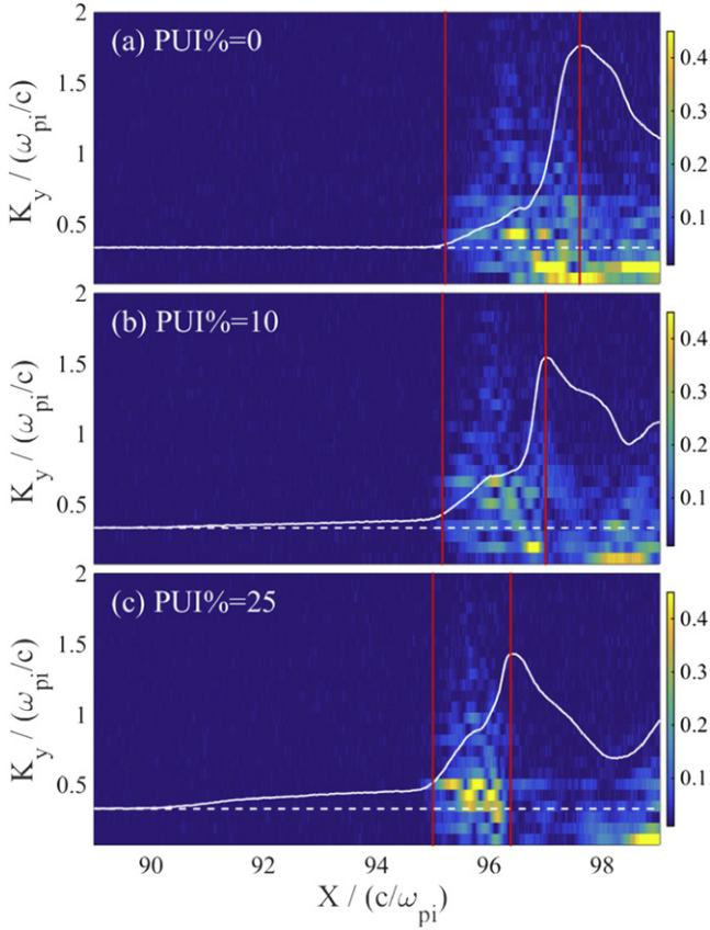
Figure 2. Power spectrum of the fluctuating magnetic field B across the shock with 0%, 10%, and 25% PUIs (from top to bottom) at t = 4 \Omega_{ci}^{-1} . The color shading indicates the power (|B(K_y)|^2) that is obtained by Fourier transforming the values of B along the Y direction at a selected position X . The vertical red lines denote the interval of the rippling region. The profile \bar{B}/3 (averaged along the Y direction) is superimposed.
