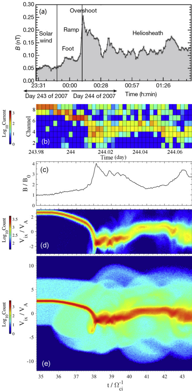
Figure 8. (a) 48 s averages of the magnetic field strength B at the TS (TS-3, after Burlaga et al. 2008). (b) Velocity distribution observed by Faraday cups on V2. Different channels correspond to different velocity ranges. The color shading shows logarithmic distributions of the current or particle count number. (c) The in situ magnetic field strength B seen by a virtual probe (VP) across the TS profiles obtained from Run C (PUI% = 25). (d) Corresponding logarithmic distributions of the ions seen by the VP across the TS. Here, the particle counts range from 40 to 5000. (e) Similar plot as in panel (d) but with a full count sensitivity (counts range from 0 to 5000). It shows the complete distribution of the total ions across the TS.
