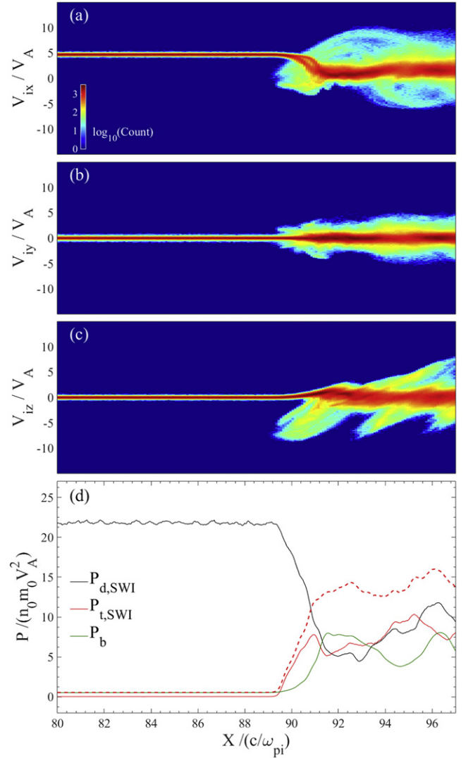
Figure 5. (a) Phase space plots ( X-V_{ix} ) of the SWIs at t = 7 \Omega_{ci}^{-1} in Run A (PUI% = 0). The color shading shows logarithmic distributions of the particle number. (b)-(c) Similar plots, but for X-V_{iy} and X-V_{iz} , respectively. (d) The dynamic pressure of SWIs (black), the thermal pressure of SWIs (red), and the magnetic pressure (green) across the shock front. The sum of the SWI thermal pressure and the magnetic pressure is also shown for reference (red dashed).
