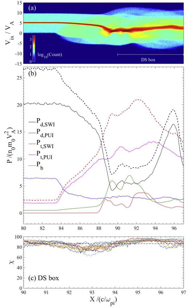
Figure 7. Same format as Figure 6, but for Run C (PUI% = 25).
