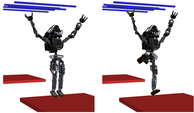
(a) Landing with a fixed mode sequence. The left toe touches the ground first (b) Landing without a pre-specified mode sequence. The right heel touches the ground first
