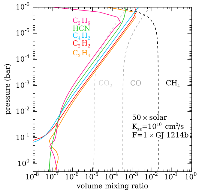
Figure 4. Carbon photochemistry for a 50\times solar metallicity model with GJ 1214b’s incident flux and K_{zz} = 10^{10} \text{cm}^2 \text{s}^{-1} . Soot precursors (solid lines) like \text{C}_2\text{H}_2 , \text{C}_2\text{H}_4 , \text{C}_2\text{H}_6 , \text{C}_4\text{H}_2 , and HCN form in the upper layers of the atmosphere where methane is dissociated by UV flux from the star. Other major carbon-bearing species are shown as dashed lines.
