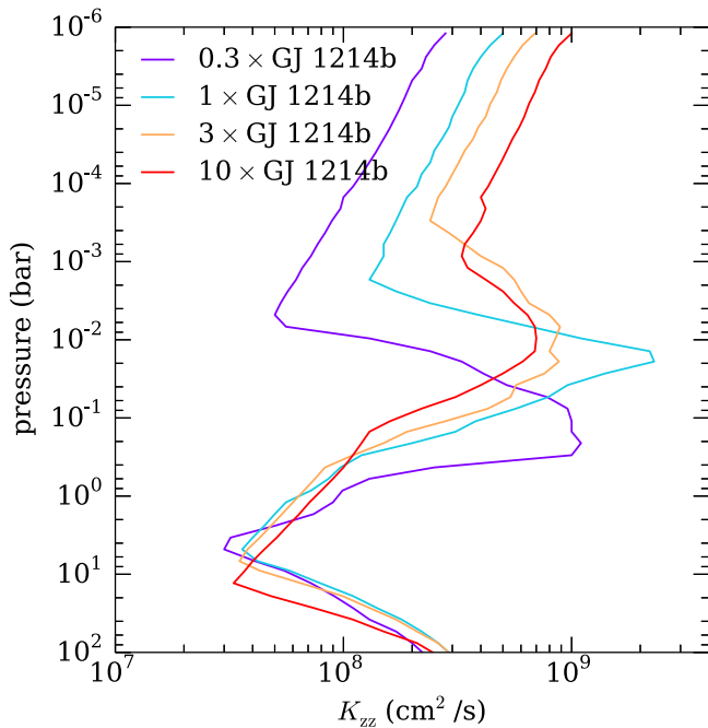
Figure 3. Eddy diffusion coefficients ( K_{zz} ) calculated within the Ackerman & Marley (2001) cloud code for models with 300\times solar composition and 0.3\text{--}10\times the incident flux of GJ 1214b.
