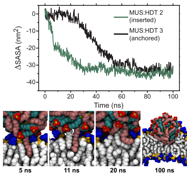
Fig. 6 NP insertion following ligand anchoring. The change in SASA is shown for the first 100 ns of a trajectory initiated from an anchored configuration (MUS:HDT 3) and compared to a trajectory from Fig. 5 (MUS:HDT 2). Snapshots from the MUS:HDT 3 trajectory are shown.
