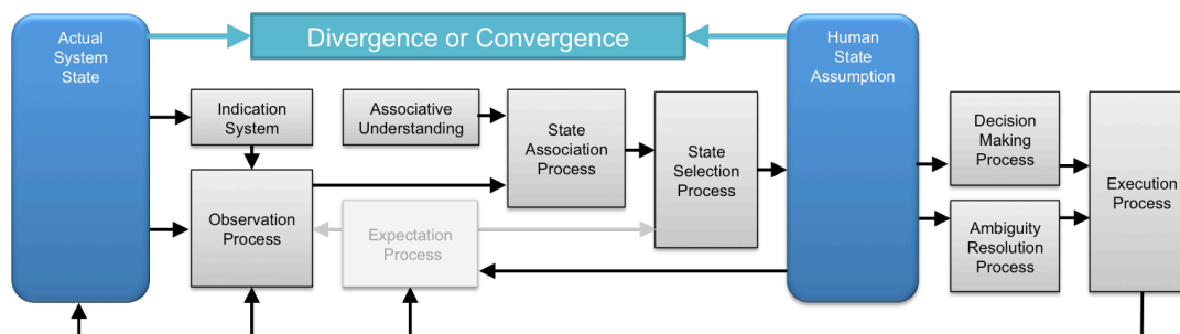
Figure 3-16. Simplified process model of divergence when confidence in expectation is low
