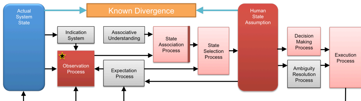
Figure 3-10. Option 2: Containment of observation process failure in the association process
