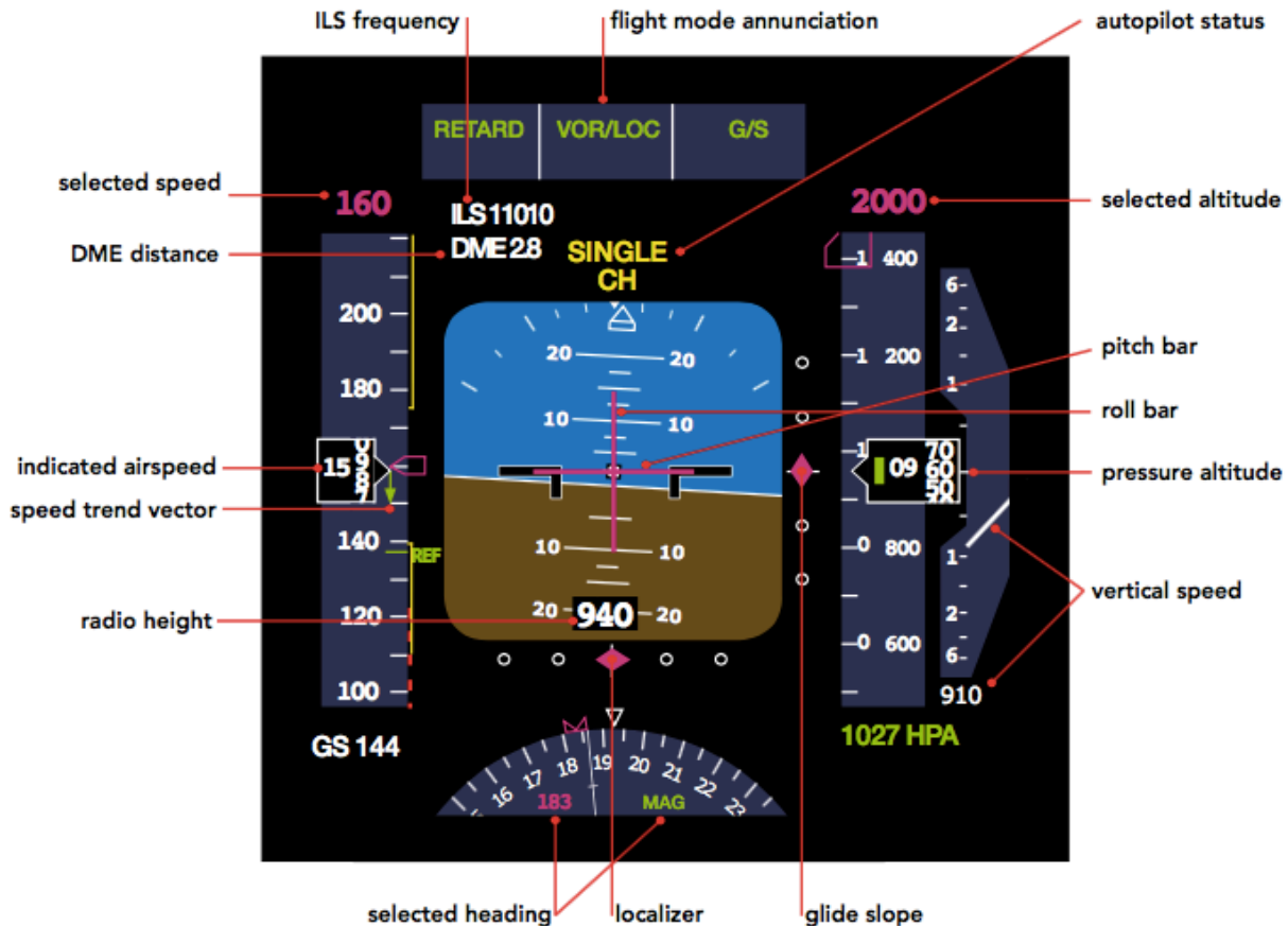
Figure 4-3. Example primary flight display in the B777 (Dutch Safety Board, 2010)
