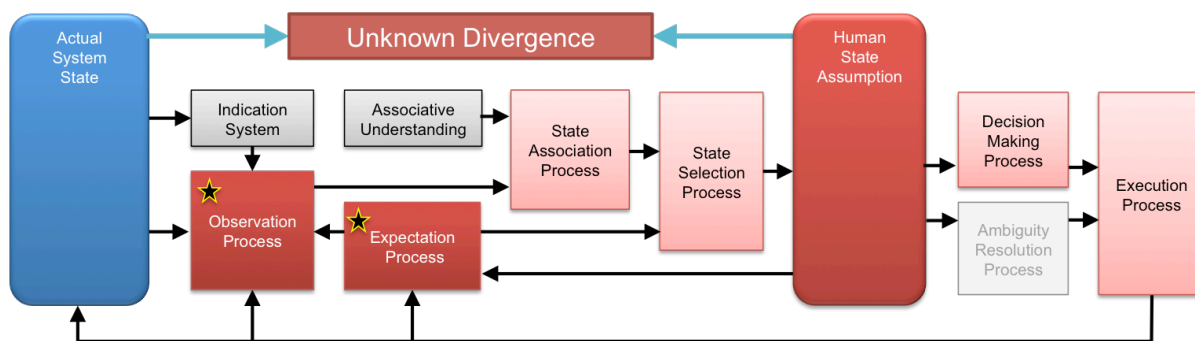
Figure 4-16. Human information processing model of divergence for Air Inter 148: Event E2 (first officer)
