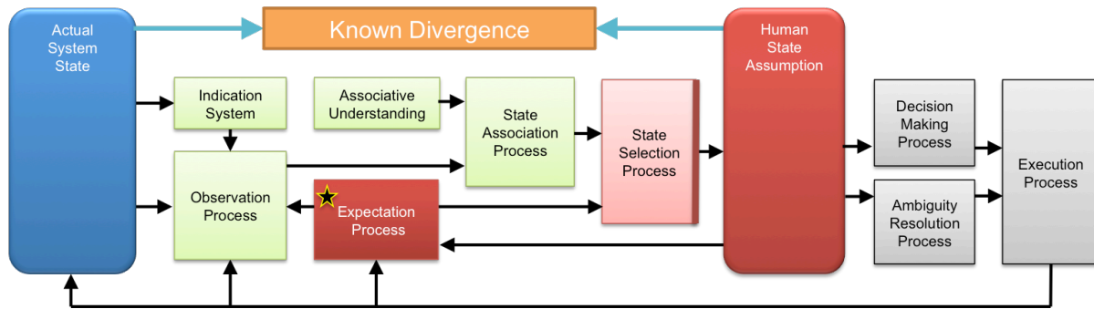
Figure 4-18. Human information processing model of divergence for Air Inter 148: Event E4
