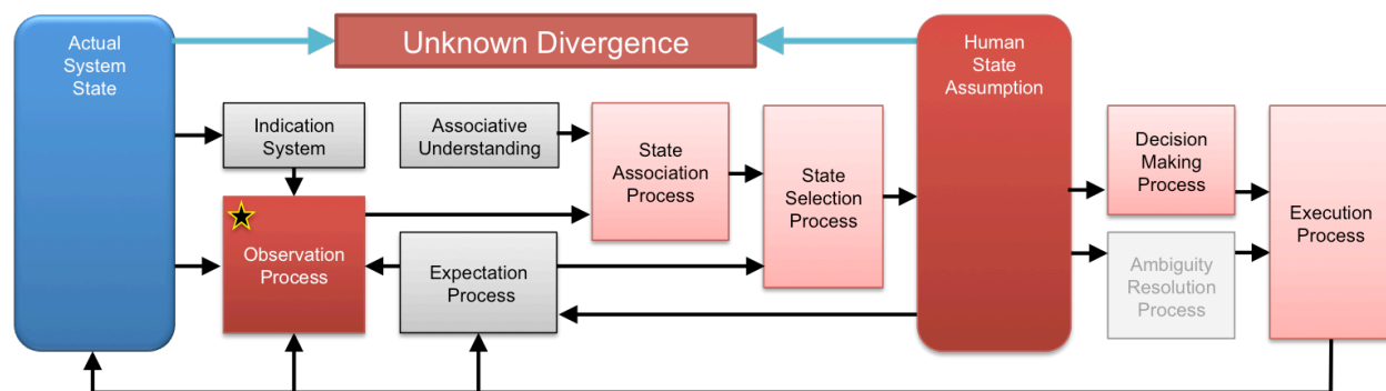
Figure 3-8. Potential propagation of observation process failure
