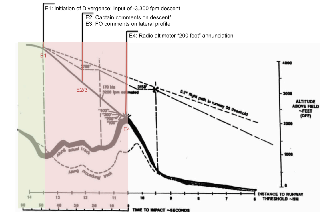
Figure 4-13. Altitude profile of Air Inter Flight 148 with divergence overlay (Bateman, 1991)
