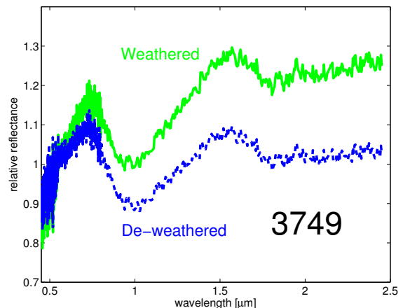
FIG. 4.— De-weathering example for the spectrum of 3749. The original spectrum (green line) is modified by Eq. (1) in a recursive way until the slope is 0.03% per \mu\text{m} (blue dashed line). This value is the average slope of the spectra of OC meteorites.
