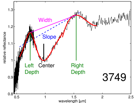
FIG. 3.— The band analysis used in our study: the red lines are the fits to the minima and peaks of the 1 \mu\text{m} absorption band. This example is for the asteroid 3749.
