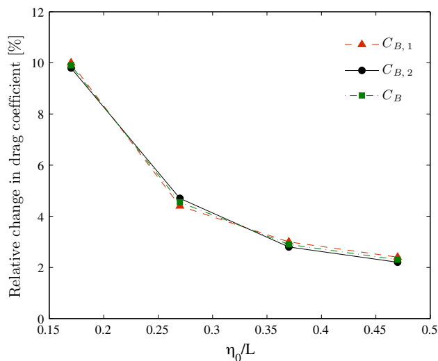
Fig. 6 Individual and combined drag coefficients for two parallel bodies, with \xi = 0 and 0.17 < \eta_0/L < 0.47 . Based on figure 6 of [38]
