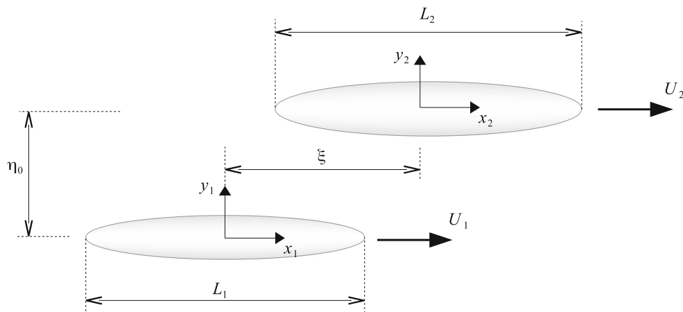
Fig. 1 Two slender bodies of lengths L_1 and L_2 separated by a lateral distance \eta_0 and a longitudinal distance \zeta(t) , moving with velocities U_1 and U_2 , respectively
