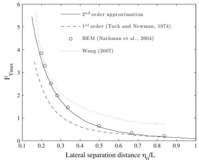
Fig. 4 Nondimensional peak lateral forces F_{Ymax} on body 1 as a function of its normalised lateral separation \eta_0/L , with \xi = 0 , \epsilon = 0.1 , and \epsilon < \eta_0/L < 1
