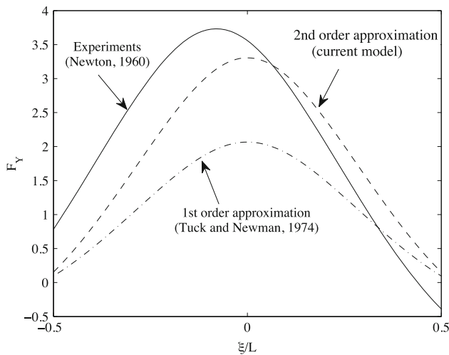
Fig. 5 Lateral forces on two ships, F_Y = Y_{\text{Newton}}/(\text{tons}/10(\text{knot})^2) (the original figure was given by Newton [2])
