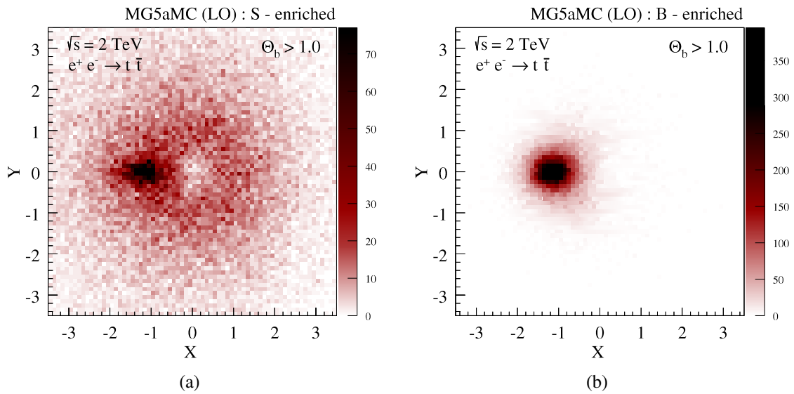
FIG. 11. The same as Figs. 7(a) and 7(b), but applying our analysis strategy on e^+e^- \rightarrow t\bar{t} events at \sqrt{s} = 2 TeV.
