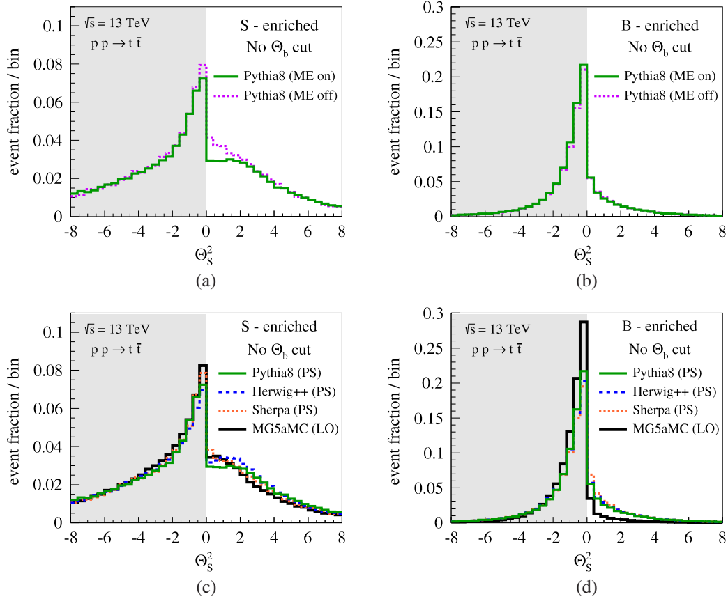
FIG. 10. The same as Figs. 8(a), 8(b), 8(c), and 8(d), but without a cut on \Theta_b .
