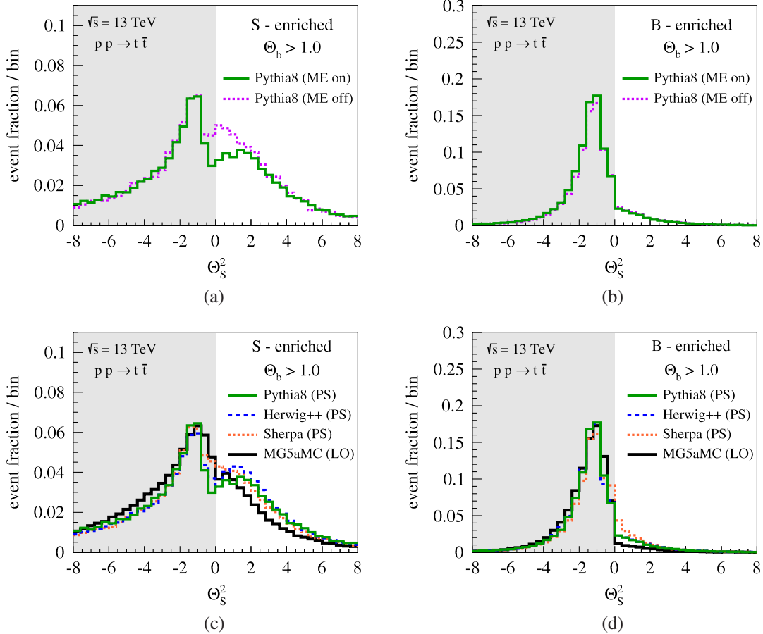
FIG. 8. Realistic distributions for \Theta_S^2 = \text{sgn}(X)(X^2 + Y^2) in 13 TeV LHC collisions, for the (left column) S -enriched and (right column) B -enriched samples. Here, a cut of \Theta_b > 1.0 has been applied; see Fig. 10 for distributions without this cut. (Top row) Turning ME corrections off and on in PYTHIA. Restricting one's attention to \Theta_S^2 \in [0, 1] for the S -enriched sample, one sees qualitatively the same dead cone physics as in Fig. 3(a). ME corrections have a negligible impact for the B -enriched sample. (Bottom row) Comparing the PS generators to LO fixed-order calculations. While each generator shows some evidence for a dead cone suppression, the quantitative behavior is noticeably different.
