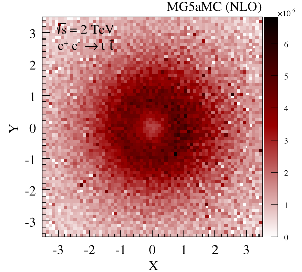
FIG. 1. Idealized gluon radiation pattern for e^+e^- \rightarrow t\bar{t} at \sqrt{s} = 2 \text{ TeV} , showing the expected dead cone suppression at the origin. This is a NLO calculation with up to two additional partons in the final state. To define the effective t^* \rightarrow tg kinematics, the gluon corresponds to the sum of emissions within the top hemisphere, imposing a cut of E_g > 50 \text{ GeV} . The X and Y coordinates are then normalized such that the dead cone peak is at X^2 + Y^2 \simeq 1 .
