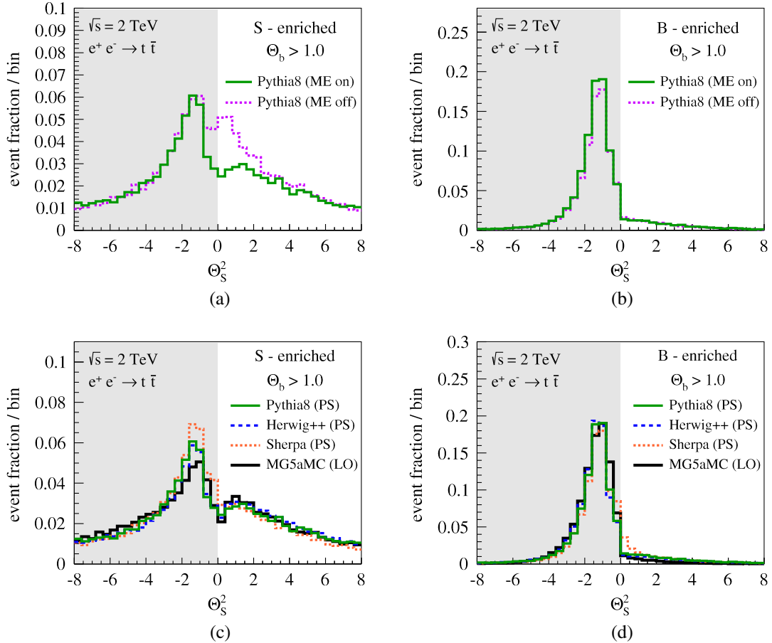
FIG. 12. The same as Figs. 8(a), 8(b), 8(c), and 8(d), but applying our analysis strategy on e^+e^- \rightarrow t\bar{t} events at \sqrt{s} = 2 \text{ TeV} .
