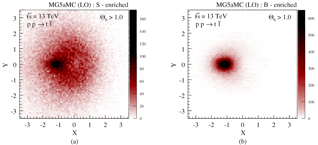
FIG. 7. The same as Figs. 6(a) and 6(b), but applying a cut on the b quark candidate of \Theta_b > 1.0 . The dead cone effect at \Theta = 0 is noticeably enhanced in the S -enriched region without sculpting a feature in the B -enriched region.
