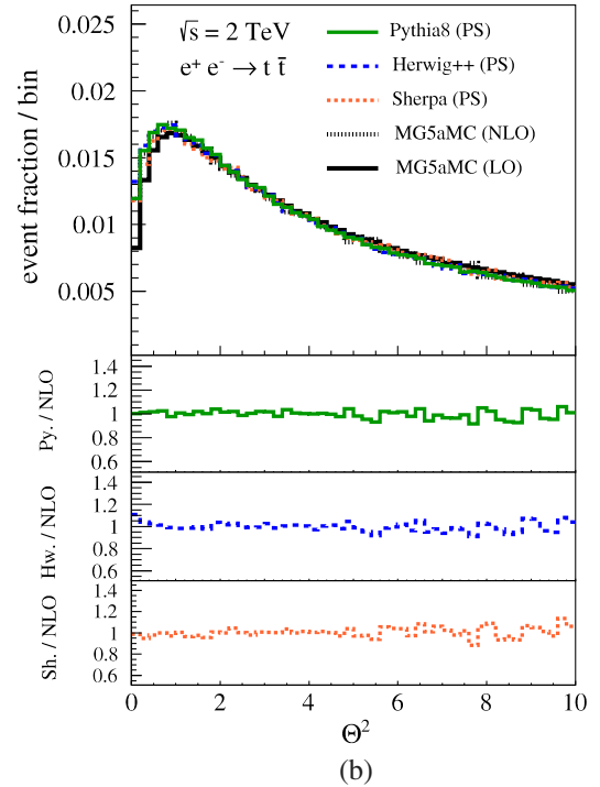
FIG. 3. The same as Fig. 2, but now considering PS predictions. (a) Turning ME corrections off and on in PYTHIA. With ME corrections off, an erroneous collinear peak is seen at \Theta^2 = 0 . With ME corrections on, the dead cone is apparent for \Theta^2 \lesssim 1 . (b) Comparing PYTHIA, HERWIG, and SHERPA PS generators to LO and NLO fixed-order calculations.
