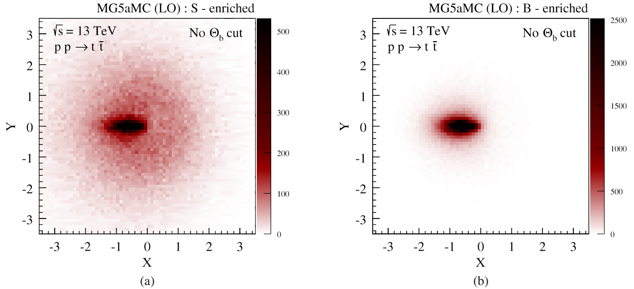
FIG. 6. Realistic angular distribution for gluon radiation in 13 TeV LHC collisions at LO. The event is rotated such that the reconstructed top flight direction is at (X, Y) = (0, 0) and the b jet points along the negative X axis. (a) The S -enriched region ( m_{b\ell\nu} \in [170, 200] GeV), showing a disk of top FSR within \Theta^2 \lesssim 1 along with contamination from b quark FSR at X < 0 . (b) The B -enriched region ( m_{b\ell\nu} < 160 GeV) where no disklike top FSR pattern is expected (or observed). See Fig. 7 for further cuts to isolate the top dead cone suppression at \Theta = 0 .
