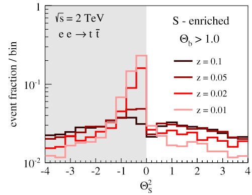
FIG. 9. The \Theta_S^2 distribution in e^+e^- \rightarrow tb\ell\nu g events at 2 TeV, for various choices of the minimum gluon energy. The cuts m_{b\ell\nu} \in [170, 200] GeV and \Theta_b > 1.0 have been applied in order to reduce direct contamination from radiation in decay. For high enough gluon energies ( z \gtrsim 0.05 ), the dead cone pattern is preserved whereas for smaller values ( z \lesssim 0.02 ), it is washed out by interference and bleed-through effects.
