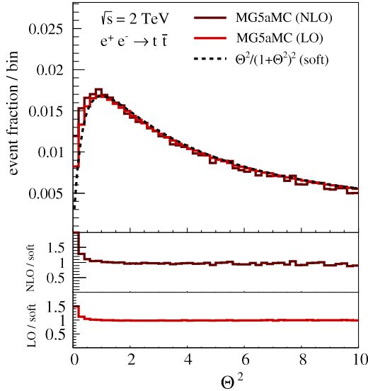
FIG. 2. Idealized distributions for \Theta^2 = X^2 + Y^2 in e^+e^- \rightarrow t\bar{t} at \sqrt{s} = 2 TeV, comparing LO and NLO calculations to the universal form in Eq. (1).
