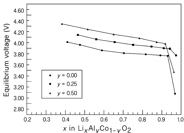
Fig. 2 Measured voltage of \text{Li}_x\text{Al}_y\text{Co}_{1-y}\text{O}_2 cathodes as a function of lithium content for three different levels of Al-doping [90]. The experimental data confirms the theoretical work of the same group predicting that Al-doping would result in higher voltages. Reprinted by permission from MacMillan Publishers Ltd: Nature [98], copyright 1998
