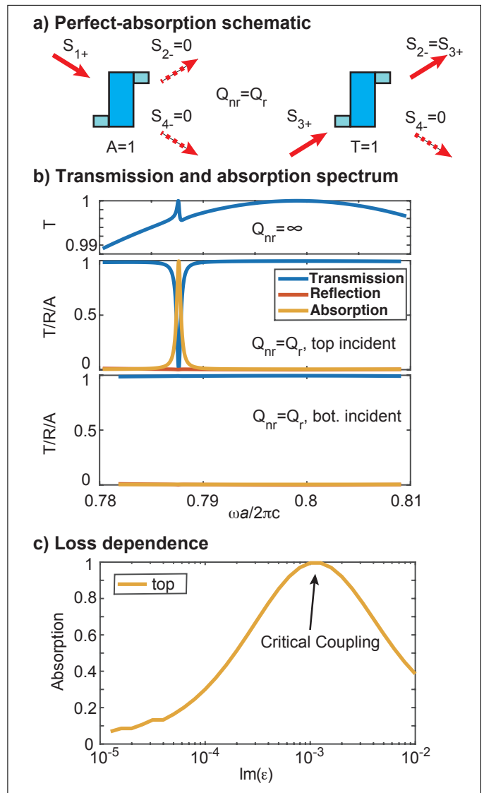
FIG. 4. Perfect absorption with single-sided illumination and no backing mirror, for single-pass absorption less than 0.5%. (a) Schematic for perfect absorption at one incident angle and perfect transmission at the opposite incident angle. (b) Transmission, reflection and absorption spectra for no loss ( Q_{nr} = \infty ) and critical loss ( Q_{nr} = Q_r ), consistent with the theoretical results in (a). (c) Loss dependence of absorption, showing near-perfect absorption for critical coupling.
