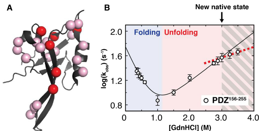
Fig. 2 Par-6 dynamics are linked to a partial unfolding process. a Residues reporting R_{ex} for PDZ 156–255 and CRIB-PDZ 130–255 (pink and red spheres). Red spheres are also globally fitted for exchange rate constants ( k_{ex} ). b Chevron rollover (gray hatched area) in the
