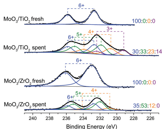
Fig. 8 XPS spectra showing the Mo (3d) binding energy region of fresh and spent MoO 3 /TiO 2 and MoO 3 /ZrO 2 from the horizontal reactor-MBMS system. The spent catalysts were retrieved at the end of the experiments shown in Fig. 3. The ratios displayed correspond to the proportion of oxidation states Mo 6+ , Mo 5+ , Mo 4+ , and Mo 3+ respectively.
