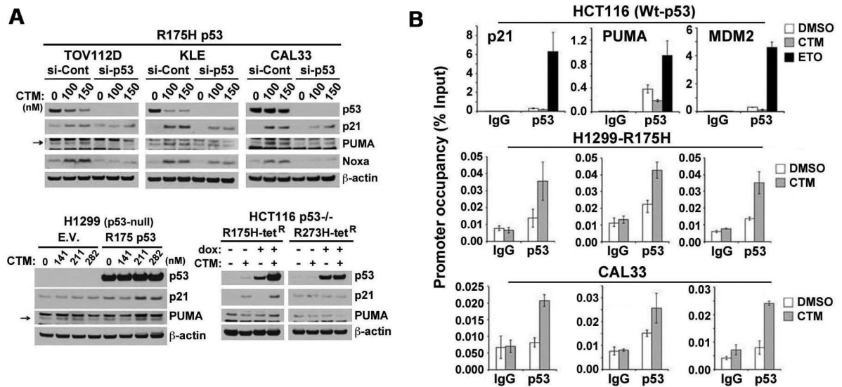
Figure 3. Mutant p53 reactivation effect of CTM is mediated through p53 R175H
