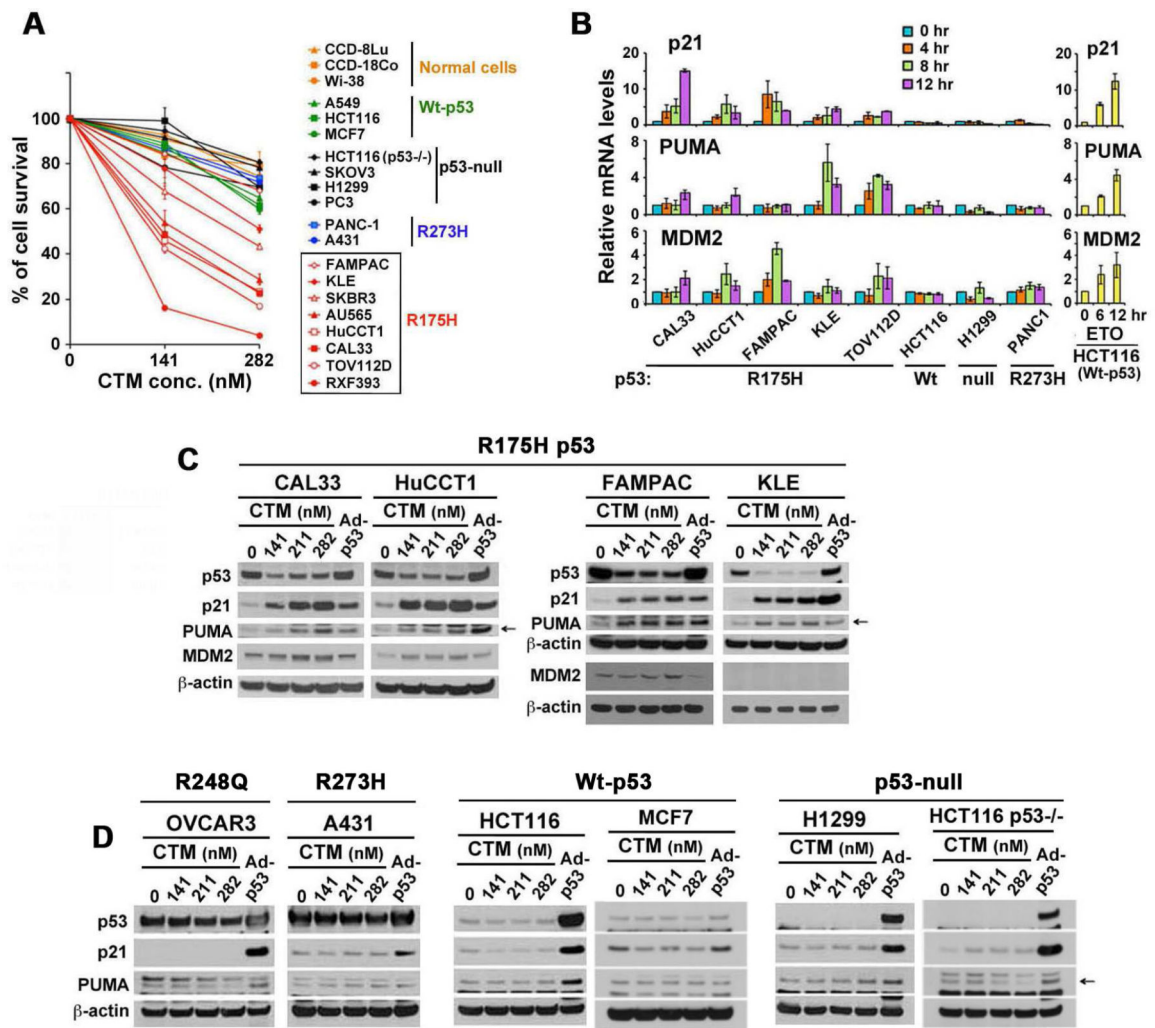
Figure 2. CTM preferentially suppresses cancer cells with p53 R175H and induces p53 target genes
