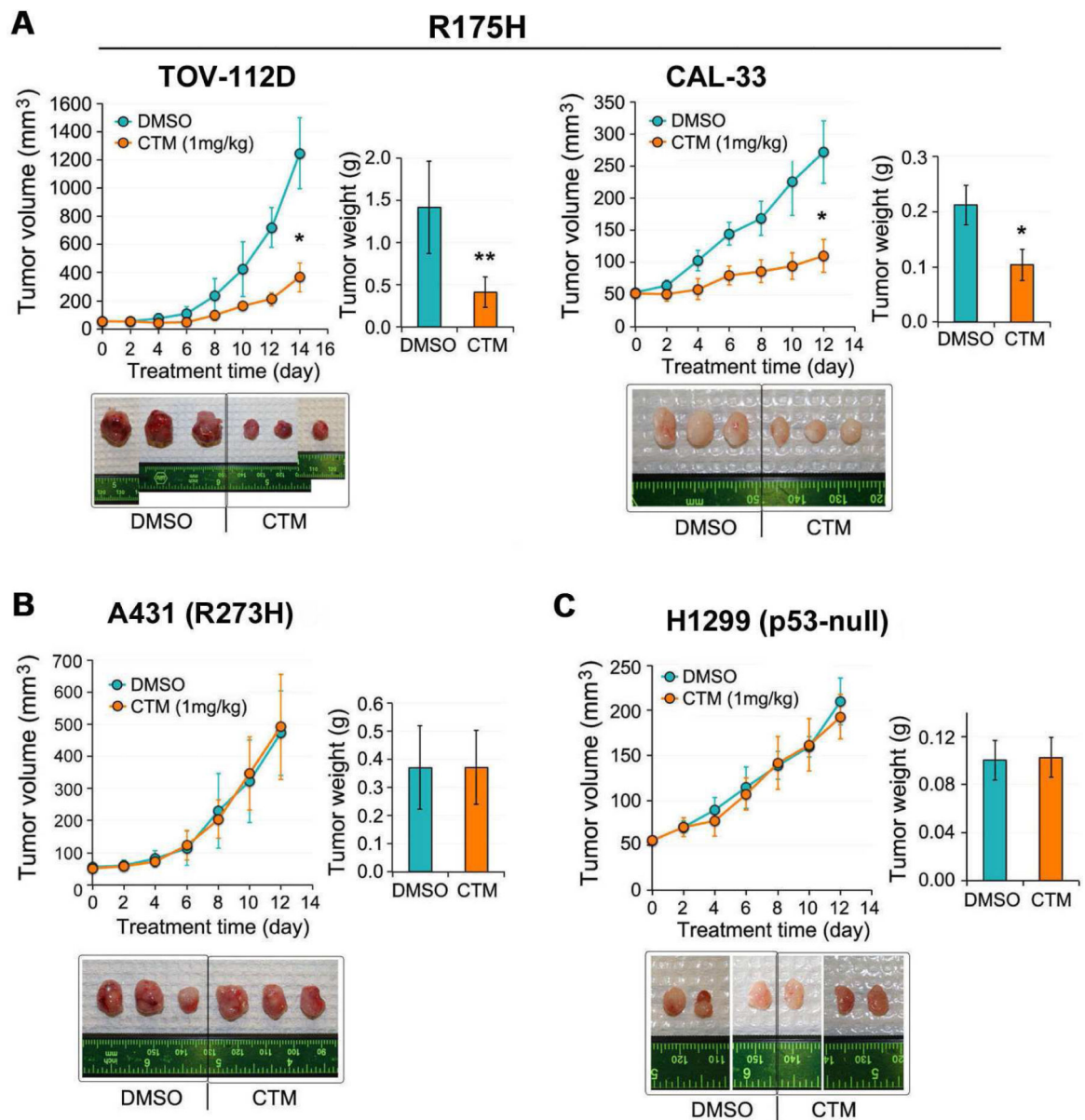
Figure 5. CTM suppresses tumor growth in vivo in a p53 R175H mutant dependent manner Various types of p53 cells were used for xenograft model-(A) TOV-112D (p53-R175H) and CAL-33 (p53 -R175H), (B) A431 (p53-R273H), (C) H1299 (p53-null). Tumors were allowed to grow to 50 mm 3 before intraperitoneal injection of DMSO or CTM at 1 mg/kg/day for indicated days. Tumor volume and weight were measured. Examined mice numbers are as follows: TOV-112D (DMSO control: n=7, and CTM-treated: n=6), CAL-33 (DMSO control: n=9, and CTM-treated: n=9), A431 (DMSO control: n=6, and CTM-treated: n=6), H1299 (DMSO control: n=8, and CTM-treated: n=8). Data shown are mean \pm S.D. Student's t -test, * P < 0.001 , ** P < 0.005 .
