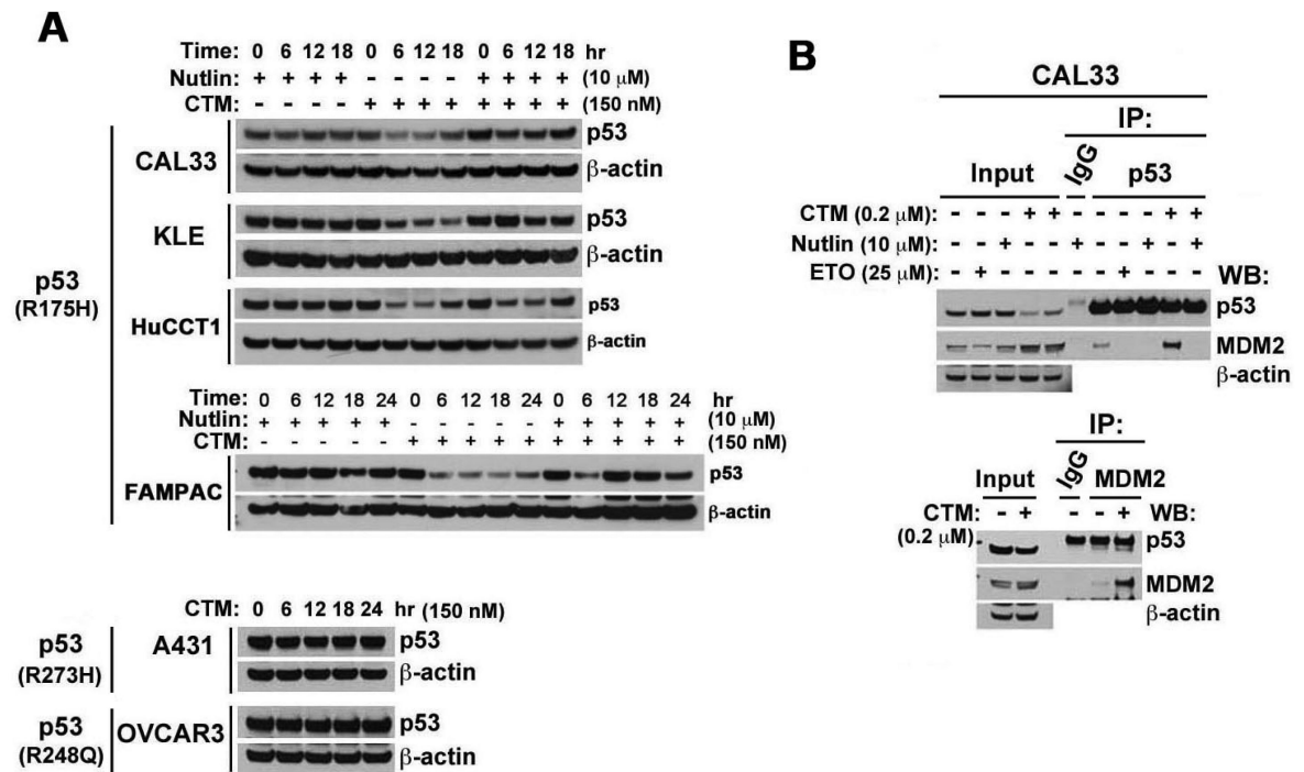
Figure 4. CTM restores p53 wild type-like properties in mutant p53 R175H
