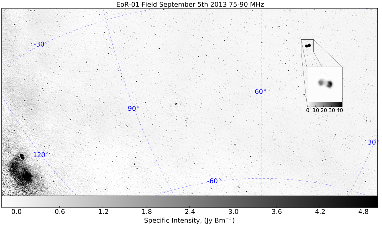
Figure 4. A deep image of the MWA “EoR-01” field centered at (R.A.(J2000) = 4^h0^m0^s and decl.(J2000) = -30^\circ0'0'' ), derived by stacking restored multifrequency synthesis Stokes XX and YY images produced by WSClean on Band 1. The dominant source in our field is Fornax A (detailed in the inset) whose structure is well recovered in imaging. Pictor A is also present at the center of the image (at \sim 30\% beam) along with the diffuse Puppis and Vela supernova remnants on the left.
