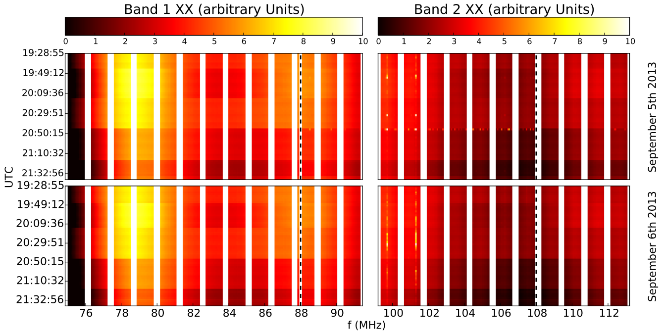
Figure 14. Dynamic spectra of the square root of a representative tile autocorrelation. Note the different color bars for the two frequency bands since Band 1 evolves more steeply in frequency than Band 2. The autocorrelations exhibit repetitive structure in time from night to night with smooth time variations occurring as the sky rotates overhead and steep transitions occurring every \approx 30 minutes due to changes in the analogue beamformer settings as the antennas track the sky. Limited RFI is plainly visible within the FM band, especially in Band 2, and the events are consistent with the flagging events identified by cotter shown in Fig. 6.
