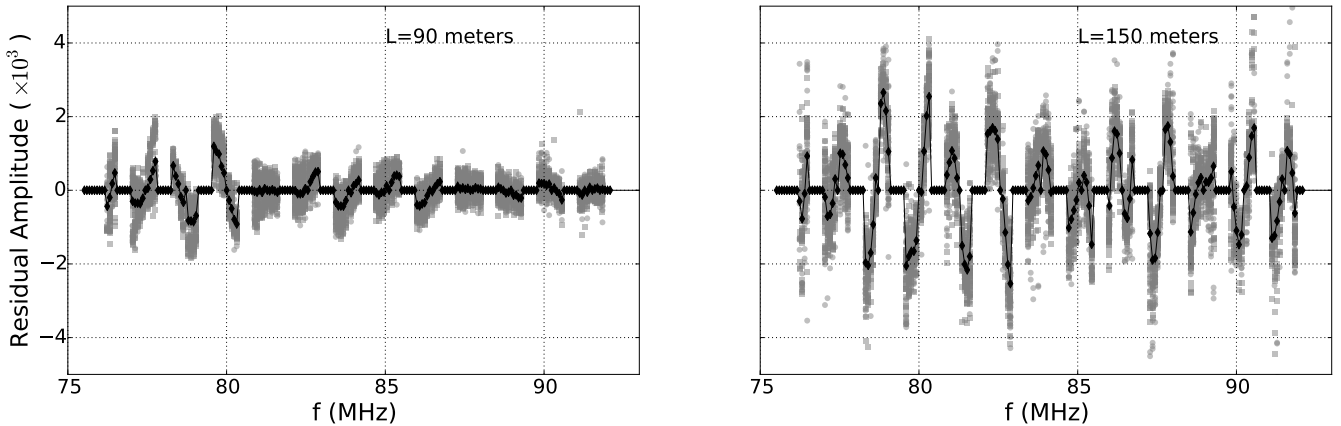
Figure 15. Left: The residuals to fitting reflection functions in our autocorrelations for all two minute time-steps in our analysis for a representative tile with a 90 meter beamformer to receiver connection (light grey points). While some scatter exists in the residuals due to fitting noise, they average to non-zero values on the order of \sim 10^{-3} (black dots). These residuals are due to mismodeling the reflections and at a lower level potentially arise from digital artifacts. Right: The same as the left but for a 150 meter cable whose reflection coefficient is \sim \times 2 as large as the 90 meter cable, leading to larger residuals due to mismodeling.
