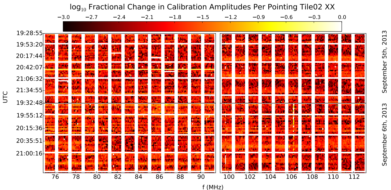
Figure 3. A false-color plot of the fractional change in our calibration amplitudes over each pointing (in which beamformer delay settings are fixed). Pointing changes are marked by the solid white horizontal lines. We see that the calibration amplitudes vary within a pointing on the order of several percent with little systematic variation. There are several coarse channel jumps on September 5th that correspond to observations in which the number of sources identified within a snapshot image were reduced (see Fig. 9). We found that these jumps corresponded to excess flagging from cotter , indicating high levels of RFI or other bad data, and dropped them from our analysis. Vertical lines from RFI are visible at 98 MHz and 107 MHz, especially on September 6th.
