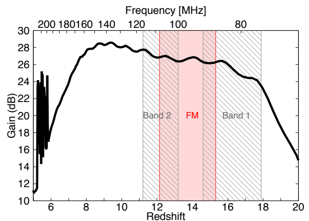
Figure 2. The autocorrelation spectrum of a single tile, showing the MWA bandpass, is plotted here (solid black line) along with the frequency ranges over which our data was taken (gray striped rectangles). Observations were performed simultaneously on two non-contiguous bands located on either side of the 88-108 MHz FM band (red shaded region) to both assess conditions within the FM band and to preserve some usable bandwidth should it have proven overly contaminated by RFI.
