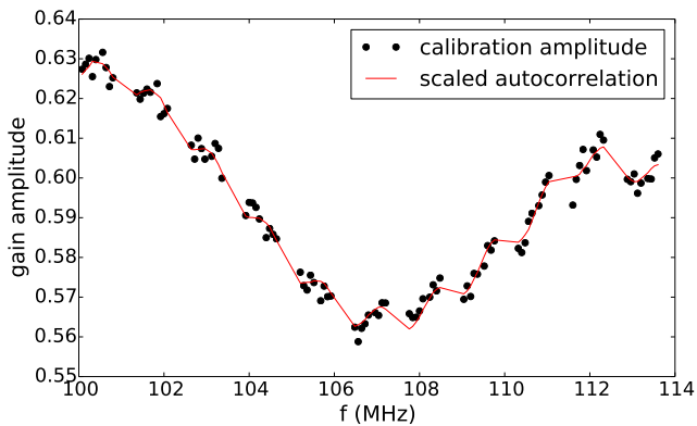
Figure 11. We show the amplitude of a calibration gain averaged over a fifteen minute pointing (black circles) along with the square root of our autocorrelations which have been scaled by a third order polynomial and a single seven meter reflection to match the calibration solution (red line). After multiplying the autocorrelations by a smooth function, they are brought into good agreement with the calibration gains.
