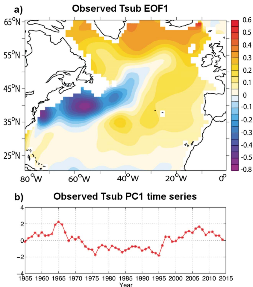
Figure 11. Variability of observed annual mean anomalies of ocean temperature at 400 m ( T_{sub} ) from an objectively analyzed ocean temperature data set [Levitus et al. , 2005]. (a) The first empirical orthogonal function (EOF1) of observed North Atlantic T_{sub} (K, 30%) for 1955–2014. (b) First principle component (PC1) time series of observed T_{sub} during 1955–2014 (normalized). Figure provided by R. Zhang (personal communication, 2015), updated from Zhang [2008].
