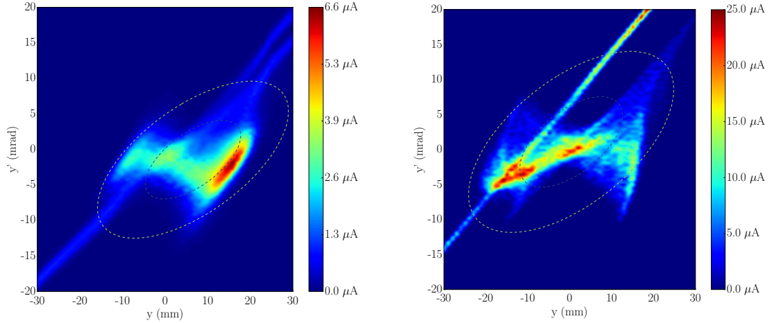
Figure 27. Comparison of measured horizontal phase space (left) and current density plot of simulated horizontal phase space (right) with SN1 at 320 A. The 'N'-shape is typical for a hollow beam and leads to significantly increased emittance. The beam energy is 55 keV in this case. The different intensity scales arise from the fact that the entrance slit of the emittance scanner was smaller than the step size.
