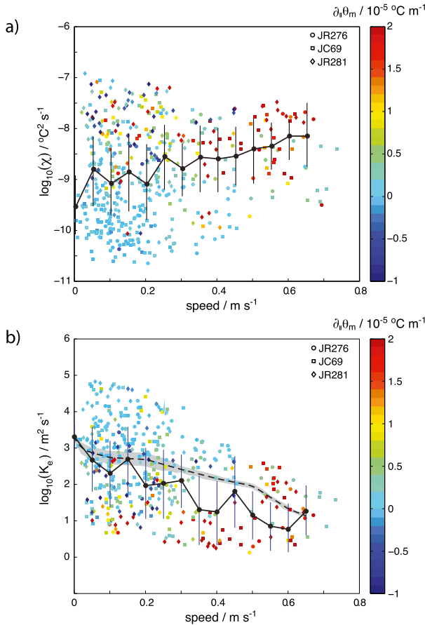
FIG. 11. Estimates of (a) \chi and (b) K_e (colored symbols, shaded by \partial_z \theta_m ) displayed as a function of LADCP-measured speed for the three SR1b section occupations with microstructure data (indicated by different symbol shapes). Averages of \log_{10}(\chi) and \log_{10}(K_e) in speed bins of 0.05 \text{ m s}^{-1} width are shown by the black circles and thick line, with the thin vertical lines denoting the standard deviation of individual \log_{10}(\chi) and \log_{10}(K_e) estimates within each speed bin. The dashed line in (b) shows the decay of K_e with increasing speed predicted by the inverse stirring suppression factor of FN10, using the mean microstructure-based K_e value at zero speed and the average altimetry-derived (depth dependent) eddy kinetic energy in each speed bin [updated from NG11]. The gray shading indicates the range of predicted K_e values associated with one standard deviation of the individual estimates of eddy kinetic energy in each speed bin.
