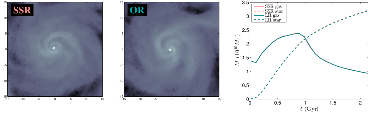
Figure 14. Simulation of the formation of an isolated magnetic disc using the two regularization schemes. The first two panels show a slice of the gas density field, while the third panel shows the time evolution of mass of stars and gas within a 15 kpc radius. Regularization does not affect the global properties of the simulation. The density scale covers -5 \leq \log_{10} \rho \leq -0.8 .
