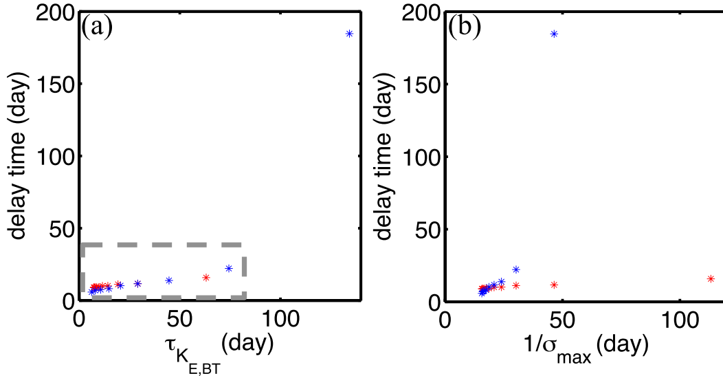
FIG. 14. (a) Scatterplot between the delay time and the barotropic eddy turnover time scale \tau_{K_{E,BT}} . (b) Scatterplot between the delay time and 1/\sigma_{\max} , where \sigma_{\max} is the maximum growth rate diagnosed using the linear stability analysis approach from Arbic (2000). The delay time here refers to the days that \langle P_E \rangle leads \langle K_{E,BT} \rangle . Red stars are results from the group of experiments with varying \delta ; blue stars show results from the group of experiments with varying vertical shear. The dashed gray box in (a) shows the parameter space where the delay time and \tau_{K_{E,BT}} roughly satisfies a linear relation.
