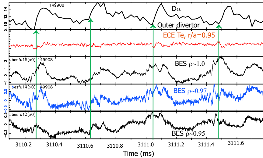
FIG. 10. Details of D_\alpha emission (top), T_e fluctuations from Electron Cyclotron Emission (second trace) and density fluctuations, from Beam Emission Spectroscopy during an I-mode period on DIII-D discharge 149908 (1.2 MA, 2.05 T). Periodic bursts of fluctuations are seen which result in small increases in D_\alpha indicating increased particle transport.
