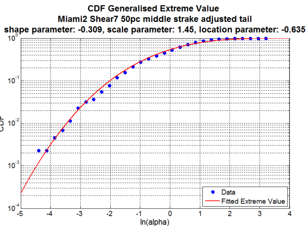
Figure 8: Adjusted GEV CDF fit Miami2 riser, 50% middle strokes.
