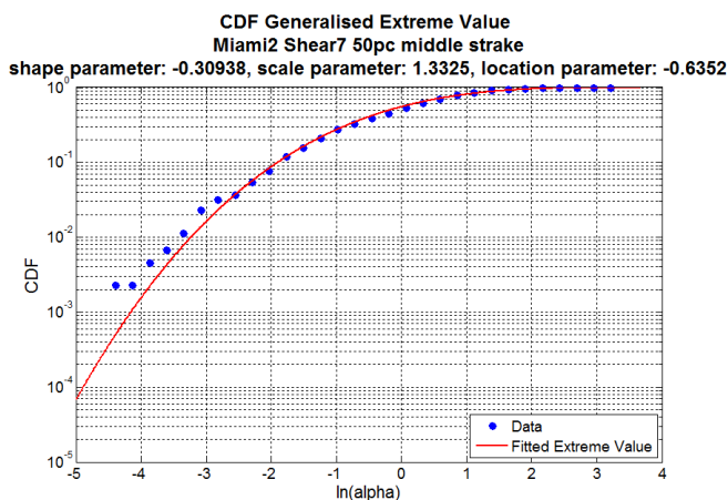
Figure 7: GEV CDF fit Miami2 riser, 50% middle strokes.
