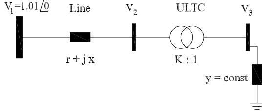
Fig. 15: A 3-bus system equipped with an ULTC
