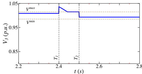
Fig. 16: Voltage multistability with the ULTC system
