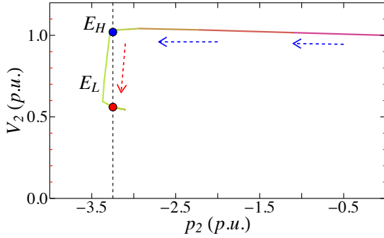
Fig. 4: The PV curve at bus 2, t < 25 s
