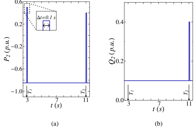
Fig. 8: Power demand level at load bus 2, t \leq 12 s
