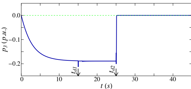
Fig. 10: The active power of load bus 3 in the load shedding induced voltage collapse
