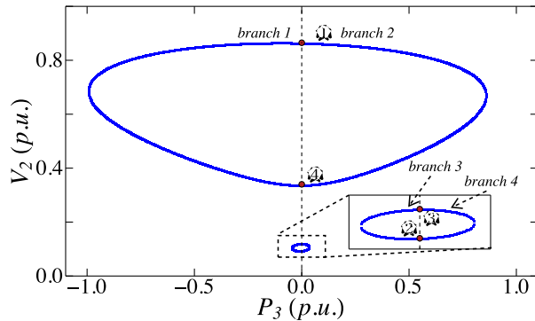
Fig. 21: P_3V_2 curves
