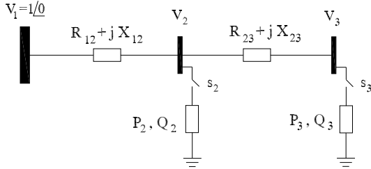
Fig. 20: A 3-bus system with fictitious switches at load buses
