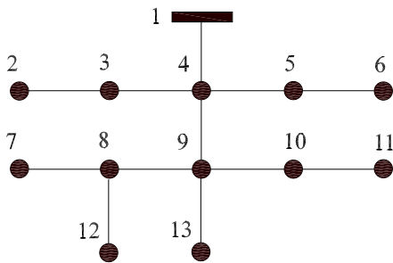
Fig. 6: The thirteen-bus feeder test case
