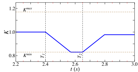
Fig. 19: The ULTC ratio during the disturbance
