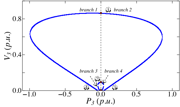
Fig. 22: P_3V_3 curves
