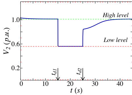
Fig. 14: Voltage at bus 2 for the large second disturbance, t \leq 45 s
