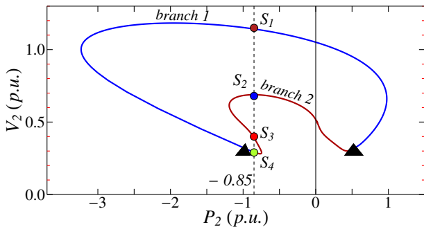
Fig. 7: The thirteen-bus feeder test case nose curve
