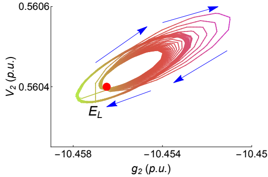
Fig. 5: The gV curve at bus 2, 25 s \leq t \leq 30 s
