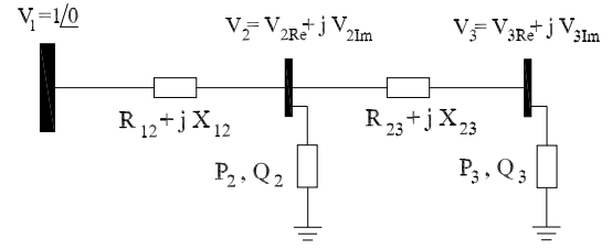
Fig. 1: A three-bus network
