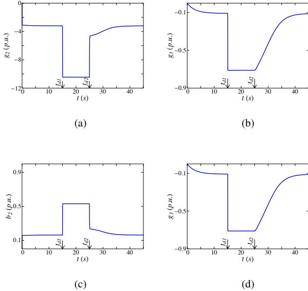
Fig. 13: The conductances and susceptances at bus 2 and bus 3, t \leq 45 s
