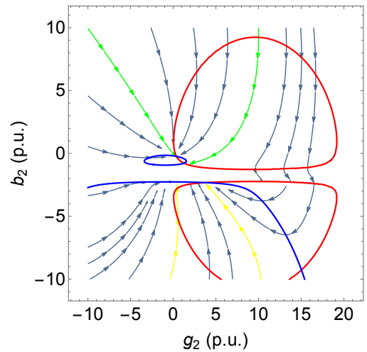
Fig. 11: The phase portrait of the 3-bus system
