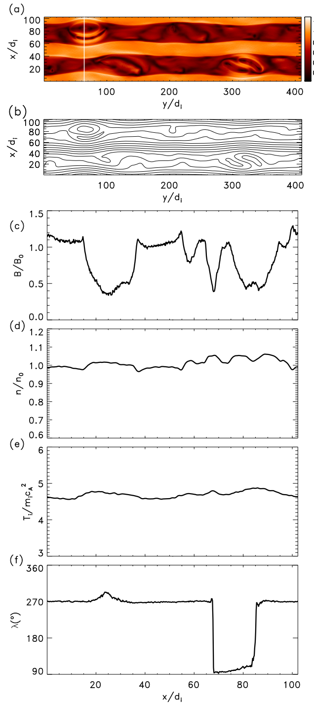
Figure 4. The late-time ( \Omega_i t = 440 ) structure of the magnetic field B in (a) and magnetic field lines in (b) over the entire simulation domain. Cuts through a remnant pair of magnetic islands along the white line in (a) showing B in (c), of the density n in (d), the ion temperature T_i in (e), and the azimuthal angle \lambda in (f).
