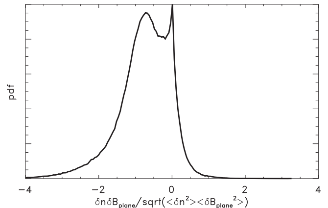
Figure 8. From the simulation a histogram of \delta n \delta B_{\text{plane}} / \sqrt{\langle \delta B_{\text{plane}}^2 \rangle \langle \delta n^2 \rangle} , where \delta n = n - \langle n \rangle , \delta B_{\text{plane}} = B_{\text{plane}} - \langle B_{\text{plane}} \rangle with n the density, B_{\text{plane}} the magnitude of the in-plane magnetic field, and \langle n \rangle and \langle B_{\text{plane}} \rangle the average over the computational domain.
