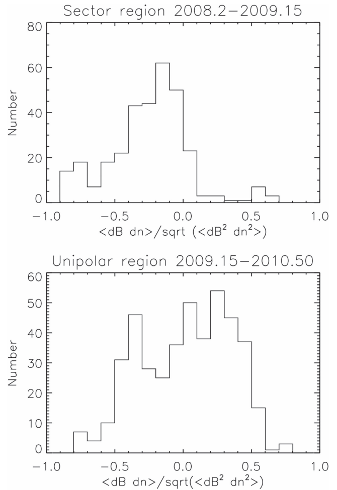
Figure 7. Histograms of \langle dBdn \rangle / \sqrt{\langle dB^2 \rangle \langle dn^2 \rangle} where dB = B - \langle B \rangle and dn = n - \langle n \rangle from Voyager 2 in the sectored region (top) and the unipolar region (bottom). We use 25-day averaging windows.
