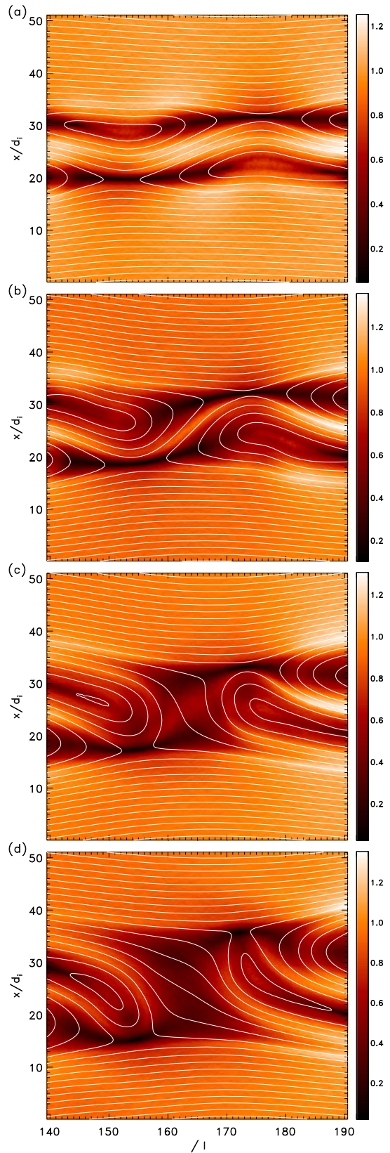
Figure 2. A blowup view of the time evolution of a pair of magnetic islands at \Omega_i t = 100, 150, 200, and 250 showing how the subdominant flux is annihilated. The magnetic field B is shown in color and the overlaid white lines are magnetic field lines. The times shown are before the islands overlap the adjacent current layer in (a), when they first intersect the adjacent current layer in (b), and when the magnetic flux in the islands is eroded in (c) and (d).
