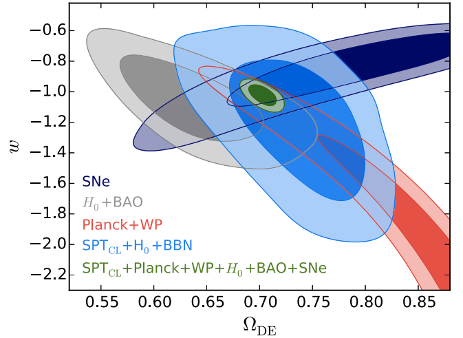
Figure 8. Comparison of different cosmological probes of dark energy. The contours show the simultaneous constraints on the present-day density of dark energy \Omega_{\text{DE}} = 1 - \Omega_m and the dark energy equation of state parameter w . Using priors on H_0 and \Omega_b h^2 , the SPT cluster data are able to simultaneously constrain the two parameters, and are in good agreement with the other probes. The other probes are sensitive to dark energy primarily through its effect on the geometry of the universe.
