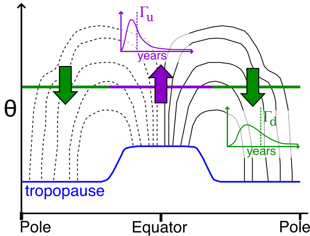
FIG. 1. A schematic diagram of the time-average circulation of the stratosphere and the overturning through one isentrope. The diabatic circulation streamfunction is sketched in the black contours. The upwelling region of the isentrope is purple, and the downwelling region is green. (insets) The age spectra are shown schematically for the upwelling and downwelling air, along with the means, \Gamma_u and \Gamma_d . Based on a similar diagram in Vaugh and Hall (2002) .
