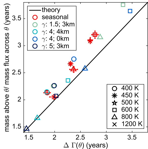
FIG. 7. The ratio of mass above an isentrope to mass flux through an isentrope vs the difference between downwelling and upwelling age of air on the isentrope. The green and blue points are averages from the last 2000 days of perpetual-solstice runs, as described in Table 1. The red points are the average of 50 annual averages from the seasonally varying run with 4000-m topography and lapse rate of 4 \text{ K km}^{-1} . The error bars are one standard deviation of the annual averages. The black line shows the one-to-one relationship predicted by the theory, and the different symbols are different isentropic levels.
