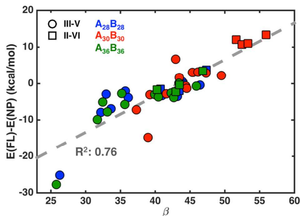
Figure 10. Relationship of relative energy per pair of AB atoms in kcal/mol of A_{28}B_{28} (blue), A_{30}B_{30} (red), and A_{36}B_{36} (green) fullerenes referenced against the A_{36}B_{36} spherical nanoparticles from III-V (circles) and II-VI (squares) materials with a descriptor \beta which is a linear combination of sum of covalent radius of A and B atoms, total energy penalties of four-, five-membered rings, and number of six-membered rings (the form of \beta is shown in text). A best-fit line (gray dashed) is also shown.
