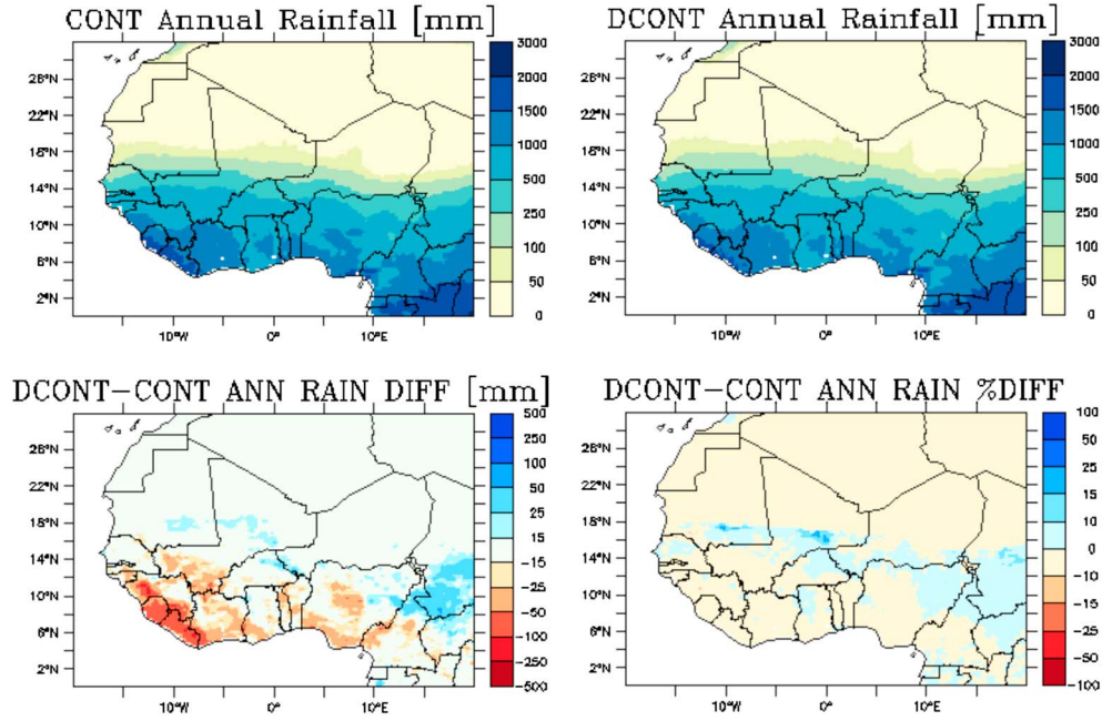
Figure 7. Same as Figure 6 but for annual rainfall (mm/yr). Also plotted is percent difference in annual rainfall between DCONT and CONT. Note that annual rainfall under 100 mm is masked from difference plots.
