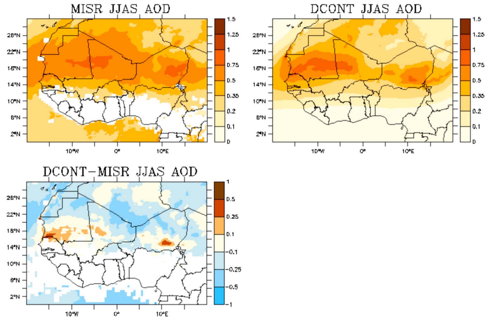
Figure 3. Average JJAS daily AOD for MISR observations and DCONT simulation. Also plotted is model bias (DCONT-MISR) for simulated AOD.
