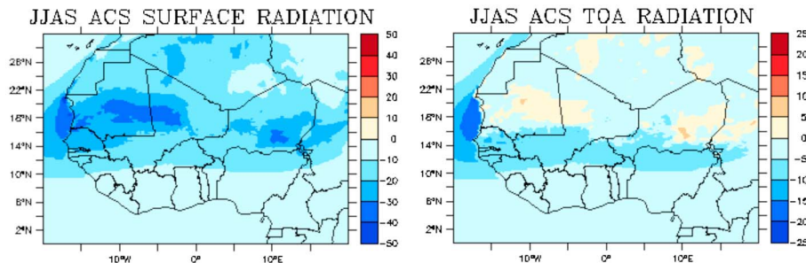
Figure 5. Same as Figure 3 but for DCONT’s clear sky (cloud effects removed) surface net shortwave radiation and top of atmosphere (TOA) net shortwave radiation both in ( \text{W}/\text{m}^2 ).
