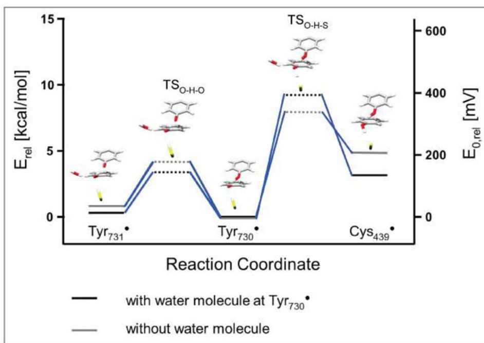
Fig. 5. Energy level diagram including the transition states for the PCET pathway residues Y_{731} - Y_{730} - C_{439} . The reaction coordinate was investigated using the large models 7 and 8 (Table 2), with and without the water molecule. Shown are only parts of the optimized structures of model 7 (with water molecule).
