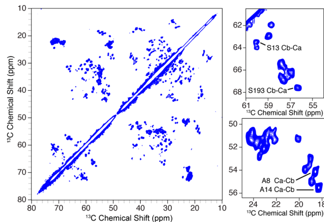
Figure 2. ^{13}\text{C} – ^{13}\text{C} RFDR MAS correlation spectrum of [U\text{-}^{13}\text{C},^{12}\text{C}\text{-FLY},^{15}\text{N}]\text{VDAC} in DMPC lipid bilayer 2D crystals. Assignments for A8, S13, A14, and S193 are labeled in expansions of the spectrum (right). Experimental parameters were as follows: \tau_{\text{mix}} = 1.3 ms, \omega_r/2\pi = 12.5 kHz, \omega_{\text{OH}}/2\pi = 750 MHz, 32 scans per t_1 slice, and a 2.5 s recycle delay for a total experiment time of \sim 16 h.
