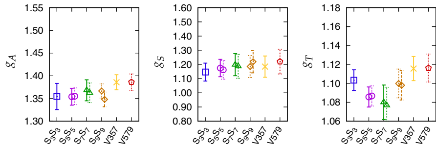
FIG. 17. Comparison of the estimates of the unrenormalized charges obtained using a 2-state fit with \langle 1|O_T|1\rangle = 0 to all the t_{\text{sep}} = 12 data. The data point with solid error bars are from R2, dotted from R3 and dashed from R4.
