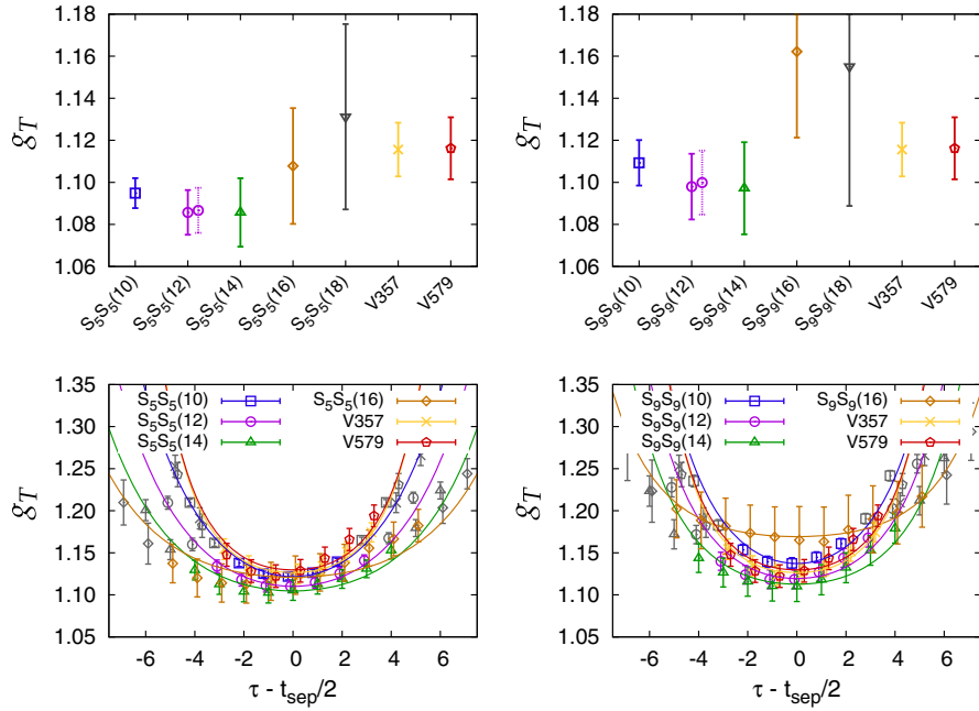
FIG. 18. Comparison of estimates of the unrenormalized g_T from the S_5 S_5 data (left) and the S_9 S_9 data (right) for different values of t_{\text{sep}} with V357 and V579. The rest is the same as in Fig. 16.
