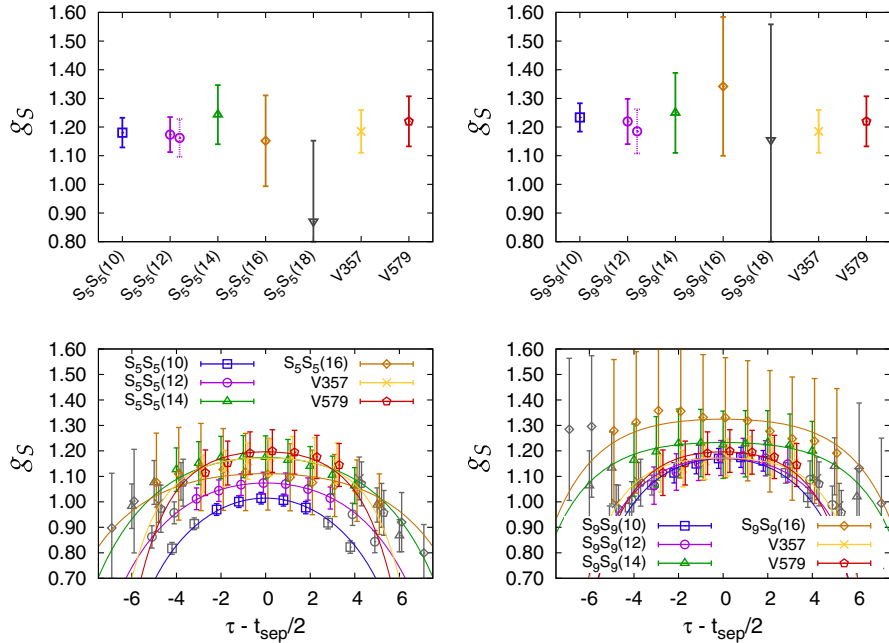
FIG. 19. Comparison of estimates of the unrenormalized g_S from the S_5 S_5 data (left) and the S_9 S_9 data (right) for different values of t_{\text{sep}} with V357 and V579. The rest is the same as in Fig. 16.
