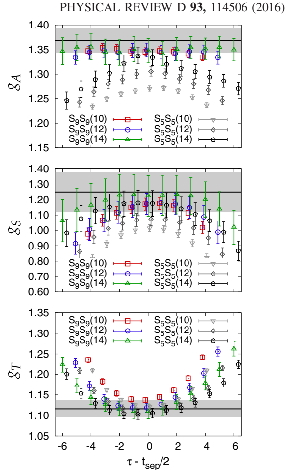
FIG. 12. Ratio plot comparing the statistical errors and excited-state contamination in the three unrenormalized isovector charges between runs R1 ( S_5S_5 ) and R4 ( S_9S_9 ) for values of t_{\text{sep}} = 10, 12, 14 shown within parentheses. The error band and the solid line within it are the t_{\text{sep}} \rightarrow \infty results of fits to the S_9S_9 data. In most cases, the data with the two different smearings start to overlap by t_{\text{sep}} = 14 . The errors in the data with t_{\text{sep}} = 16 , shown in Fig. 13, are too large to confirm the convergence.
