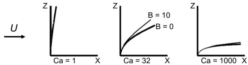
Figure 2. Blade posture predicted by Luhar model for different values of Cauchy number ( Ca = 1, 32 and 1000 ) and two values of Buoyancy parameter ( B = 0 and 10 ). In each subplot, B = 0 and 10 shown by thicker and thinner curves, respectively, as noted in the center subplot. For Ca = 1 and 1000 , the two curves essentially overlap.
