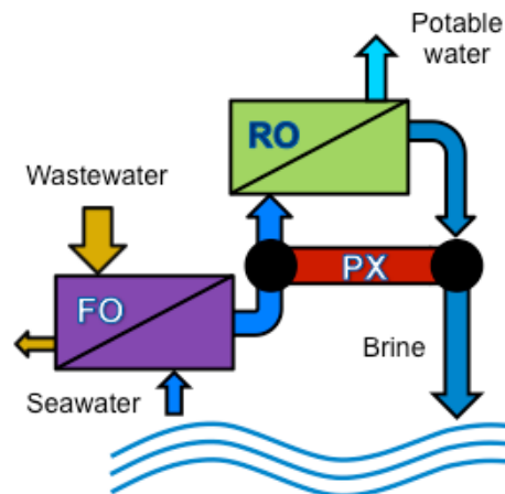
Figure 15. Schematic diagram of an FO-RO system for integrated SWRO and wastewater recovery. Water from the wastewater is extracted by osmosis through the FO process and dilutes the seawater before entering the RO process.
