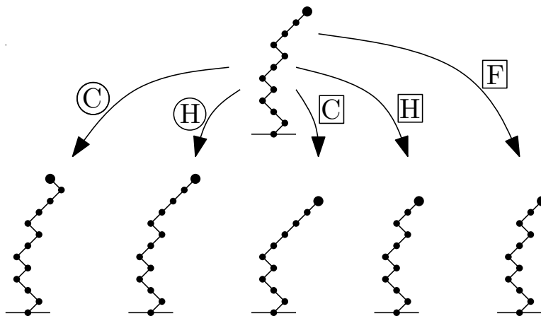
Figure 1: Above: top few elements on the stack X(-\infty, n - 1) represented by an up-left edge for each cheeseburger and an up-right edge for each hamburger. Below: top few elements of X(-\infty, n) , depending on value of X(n) . The uppermost dot above (shown slightly larger) is positioned at a location A_{n-1} = (\mathcal{D}_{n-1}, \mathcal{C}_{n-1}) describing the net change in inventory since time zero. The new uppermost dots below are positioned at locations A_n = (\mathcal{D}_n, \mathcal{C}_n) .
