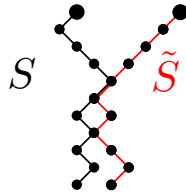
Figure 4: Upper portion of embedded stacks S \leq \tilde{S} (partially overlapping).
