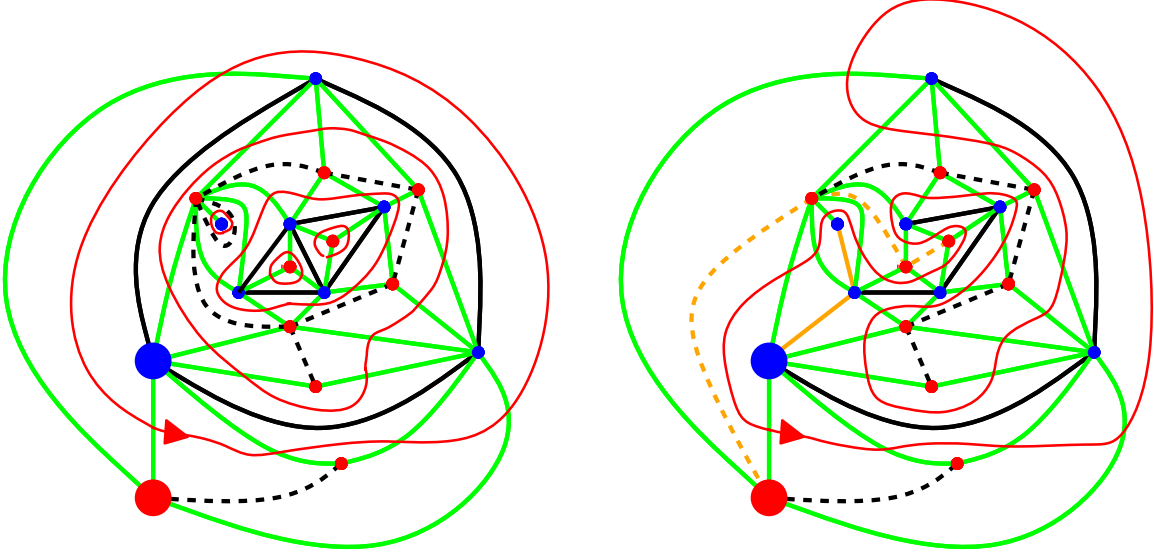
Figure 8: Left: The subset of edges does not form a spanning tree, so we obtain multiple red loops (again, each green line is crossed once). Right: a canonical way to replace some edges with dual edges, and vice versa, to obtain a spanning tree.
