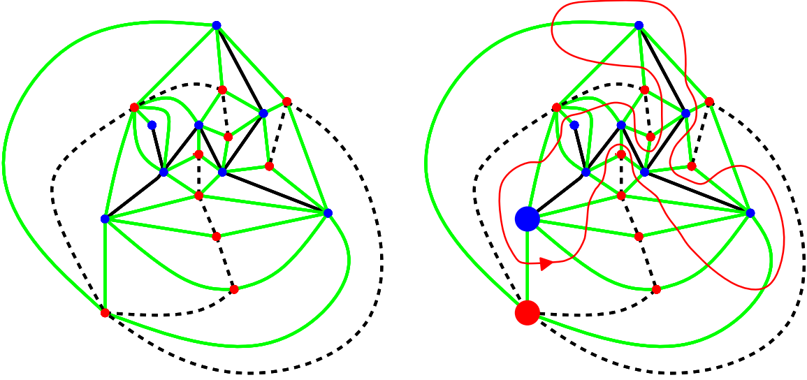
Figure 6: Left: in each quadrilateral we either draw an edge (connecting blue to blue) or the corresponding dual edge (connecting red to red). In this example, the edges drawn form a spanning tree of the original (blue-vertex) graph, and hence the dual edges drawn form a spanning tree of the dual (red-vertex) graph. Right: designate a “root” (large blue dot) and an adjacent “dual root” (large red dot). The red path starts at the midpoint of the green edge between the root and the dual root and crosses each of the green edges once, keeping the blue endpoint to the left and red endpoint to the right, until it returns to the starting position.
