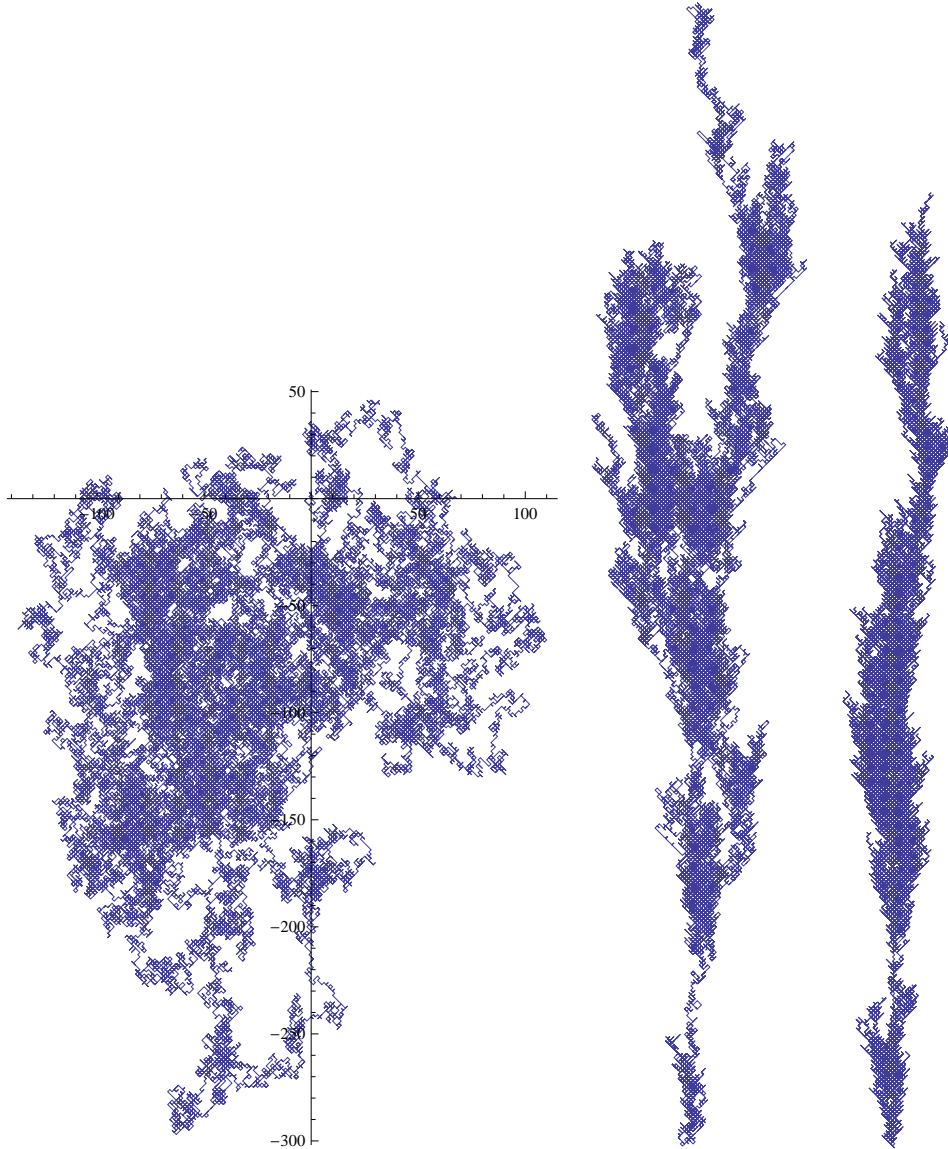
Figure 2: Sample trajectory traced by A_n = (\mathcal{D}_n, \mathcal{C}_n) as n ranges from 0 to 100000 when p = .25 (left). Similar trajectories (axes not shown) when p = .75 (middle) and p = 1 (right). In each case we use the same initial data: X(-\infty, 0) is an infinite stack alternating between burger types. In each case X(1), \dots, X(100000) are then chosen from \mu and (\mathcal{D}_n, \mathcal{C}_n) updated accordingly for n \in \{1, 2, \dots, 100000\} . As n tends to infinity, and both axes are scaled by 1/\sqrt{n} , the left trajectory tends to a two dimensional Brownian motion with variance 1 - 2p = .5 times as large in the left-right direction as the up-down direction. The middle and right trajectories tend to one-dimensional Brownian motions, concentrated on a vertical axis. (See Remark 3.17.)
