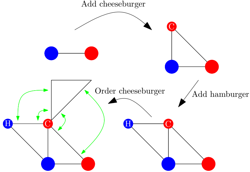
Figure 7: Start with a single edge (upper left). We will recursively construct a triangulation with two types of vertices by “exploring” triangles one at a time (c.f. Angel’s peeling process [Ang03]). At each step the outer boundary of the explored region has two edges connecting two vertices of different types: one “special edge” (to which a new triangle will be glued) and one “root edge” (the initial edge in the construction; the special edge and root edge coincide at the beginning). When a new triangle is added, there are four possibilities for its “type,” corresponding to the four symbols. Adding a triangle corresponding to one of the two “burger” symbols amounts to drawing a correspondingly colored vertex outside the surface and making a triangle by connecting it to the endpoints of the special edge (i.e., the clockwise-most boundary hamburger and the counterclockwise-most boundary cheeseburger). Adding a triangle corresponding to one of the “order” symbols amounts to making a new triangle by connecting one endpoint of the special edge to another vertex adjacent to the opposite endpoint of the special edge. At any given time in this process, the small dots on the outer boundary of the explored region correspond to burgers that have not yet been consumed. To put this somewhat fancifully, an illiterate restaurant owner armed only with triangular pieces of paper and cheeseburger and hamburger stickers could use this scheme to keep track of the day’s events, gradually constructing a surface as the day goes on.
