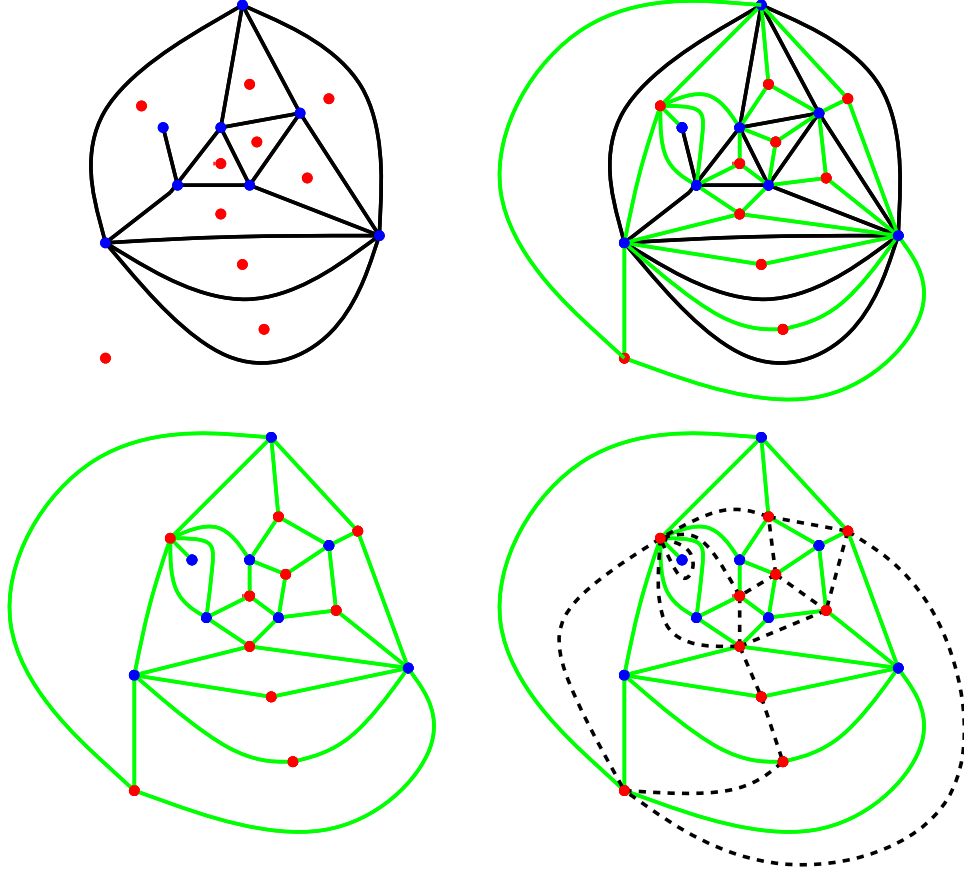
Figure 5: Upper left: a planar map M with vertices in blue and “dual vertices” (one for each face) shown in red. Upper right: the quadrangulation Q = Q(M) formed by adding a green edge joining each red vertex to each of the boundary vertices of the corresponding face. Lower left: quadrangulation Q shown without M . Lower right: the dual map M' corresponding to the same quadrangulation, obtained by replacing the blue-to-blue edge in each quadrilateral with the opposite (red-to-red) diagonal.
