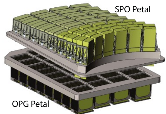
Figure 2: An Arcus channel, showing the optics petal on top with the grating petal below. Alignment and mounting hardware that connects the two petals to each other and to the optical bench are not shown for clarity.
