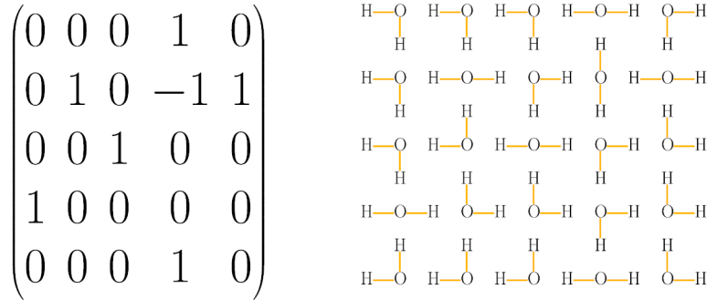
FIG. 4. An alternating sign matrix of size 5 and the corresponding configuration of the six-vertex model (square ice) with domain wall boundary condition. \mathbf{1} s in ASM correspond to horizontal molecules H-O-H and -1 s to the vertical ones.
