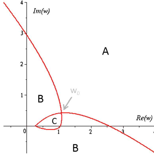
FIG. 7. Sketch of the level lines \operatorname{Re}(yw - \mathcal{F}(w; 0)) = \operatorname{Re}(yw_0 - \mathcal{F}(w_0; 0)) for y = 1 - i .
