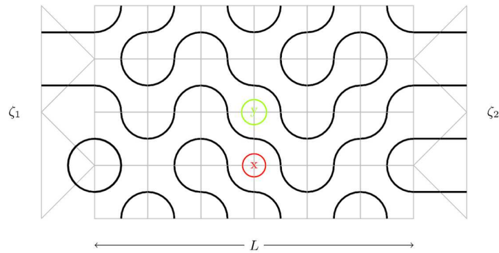
FIG. 6. A particular configuration of the dense loop model showing a path passing between two vertically adjacent points x and y .
