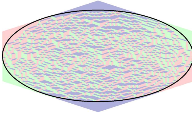
FIG. 3. A sample from uniform distribution on tilings of 40 \times 50 \times 50 hexagon and corresponding theoretical frozen boundary. The three types of lozenges are shown in three distinct colors.
