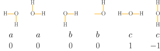
FIG. 8. Types of vertices in the six vertex model divided by groups and their correspondence to numbers in ASM.
