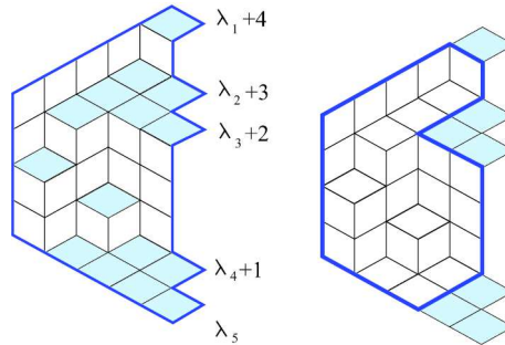
FIG. 1. Lozenge tiling of the domain encoded by signature \lambda (left panel) and of corresponding polygonal domain (right panel).
