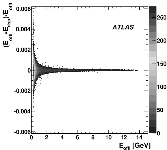
Fig. 8 Difference between the reconstructed offline energy, E_{\text{off}} , and the energy given by the DSP E_{\text{DSP}} relative to E_{\text{off}} and as a function of E_{\text{off}} (in GeV), extracted from cosmic muon runs
