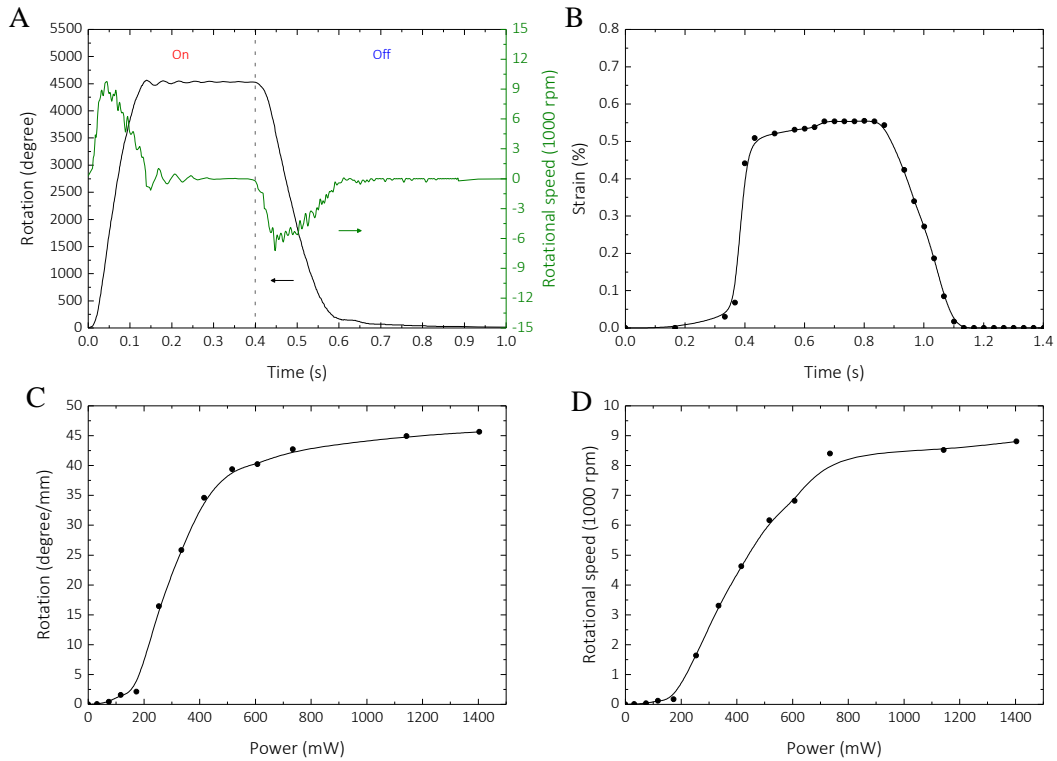
Figure 2 – (A) Response of the actuator to a square wave input with amplitude of 14 V and width of 400 ms (1.4 W). The sample had an initial inserted twist number of 75 with initial length of 250 mm. Sample was under a load of 24 MPa. (B) Tensile actuation of the actuator in (A) with the same input power. (C) Normalized torsional stroke of the actuator as a function of input power. (D) rotational speed of the actuator as a function of input power.
