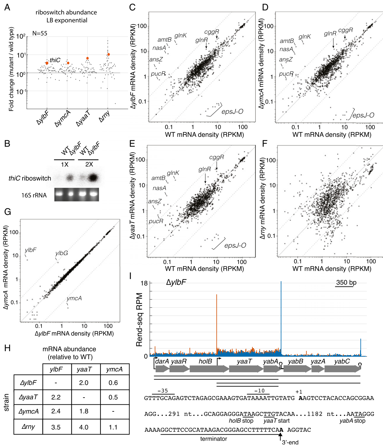
Fig. 5. Changes in RNA abundance in mutants lacking the Y-complex. (A) Fold-change in riboswitch and RNA leader abundances in mutants lacking ylbF , ymcA , yaaT , and rny compared with wild type. The number of riboswitches and RNA leaders whose expression levels are quantified in LB medium is indicated. Red dots indicate the thiC riboswitch. Only a few leaders showed greater than twofold repression, which are all regulated by CcpA ( blgF , glpD , glpF , and glpT ) and likely a consequence of transcriptional regulation. (B) Northern blot analysis showing the abundance of the thiC riboswitch in wild-type (WT) cells and cells lacking YlbF. Two dilutions of total RNA (1× and 2×) are shown with the 16S rRNA used as a loading control. The mRNA abundances for all annotated and expressed genes (>100 reads) in B. subtilis are plotted for their levels in the WT versus strains lacking ylbF (C), ymcA (D), yaaT (E), and rny (F). RNA was collected from cells in exponential phase in LB medium. Dashed lines indicate a 10-fold difference from the diagonal. RPKM, reads per 1,000 bases of gene per million bases of total reads that map to the B. subtilis genome, excluding rRNAs and tRNAs. (G) mRNA abundances for all annotated and expressed (read count >100) genes in B. subtilis are plotted for their levels in the \Delta ylbF versus \Delta ymcA . All other combinations are shown in SI Appendix, Fig. S5 . (H) mRNA levels of ylbF , ymcA , and yaaT in WT and strains lacking components of the Y-complex. (I) Rend-seq 5'-mapped (orange) and 3'-mapped (blue) read counts plotted for the yaaT region of the genome from cells lacking ylbF . In addition to the known TSS upstream of darA and the TSS in hoIB reported here, small additional peaks in 5' reads of unknown origin are present. The sequence of the 5' and 3' UTRs of yaaT and yabA are shown. Putative -10 and -35 elements of the \sigma^A consensus sequences upstream of the peak in 5'-mapped reads internal to hoIB and a putative terminator sequence upstream of the peak in 3'-mapped reads downstream of yabA are indicated. RPM, reads per million.
