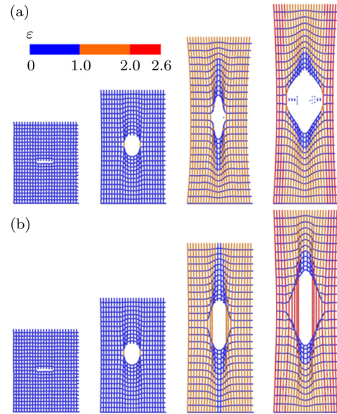
Fig. 2. Simulation snapshots of the conformations of intermediate filament networks under different applied strains (from left to right) of 0.22, 0.70, 1.50 and 2.00. (a) Intermediate filament network with crosslink strength of F_{c,0} = F_0 . (b) Intermediate filament network with crosslink strength of F_{c,0} = 0.2F_0 . Each of the filaments is colored according to its local tensile strain given by the color bar depicted in panel (a).
