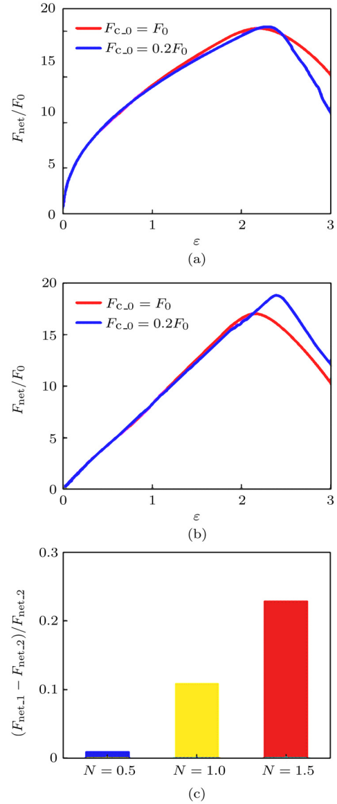
Fig. 4. Force-extension curve of networks with different mechanical characteristics under tension. (a) By using N = 0.5 in Eq. (2) to give the characteristic of strain-softening materials. (b) By using N = 1 in Eq. (2) to give the characteristic of linear elastic materials. Each of those networks is tested with two typical crosslinks strengths F_0 and 0.2F_0 . (c) Increment of the strength of the network ( F_{\text{net},1} ) with weak crosslinks ( F_{c,0} = 0.2F_0 ) comparing to that ( F_{\text{net},2} ) of the network with strong crosslinks ( F_{c,0} = F_0 ). Results of three typical materials with different N are summarized here for comparison.
