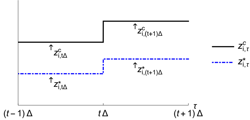
Figure 2: Illustration of z_{i,\tau}^* and z_{i,\tau}^c .
