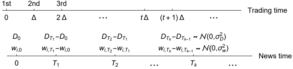
Figure 1: Model time lines. The top plot shows times of double auctions, and the bottom plot shows the news times (dividend shocks, signals of dividend shocks, and private value shocks).
