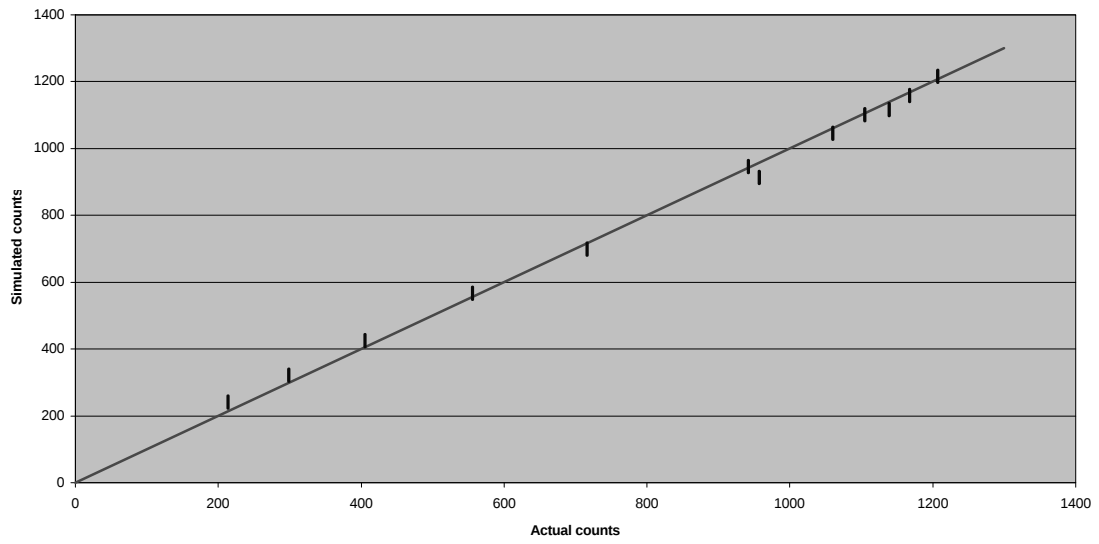
Figure 3.18: Sensor 9376A3 - West of Junction 10
