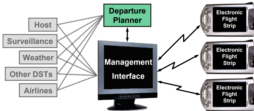
Figure 3.2: Prototype Portable Electronic Flight Strip System Architecture
