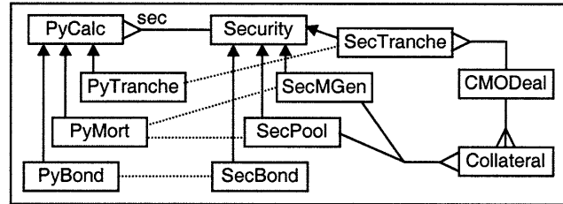
Figure 8. Polymorphic class relationships
