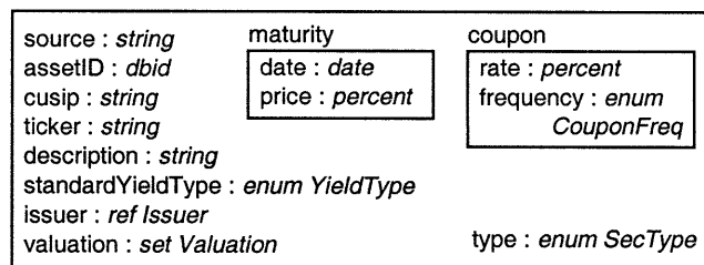
Figure 10. Generic Security class
