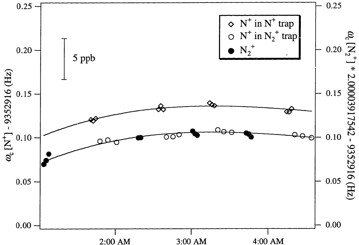
Fig. 2 Free space cyclotron frequencies for \text{N}^+ and \text{N}_2^+ . The frequency for \text{N}^+ was measured both in an \text{N}^+ trap (with 5V) and in an \text{N}_2^+ trap (with 10V). The frequency for \text{N}_2^+ has been scaled by the known ratio of M[\text{N}_2^+]/M[\text{N}^+] , so that the plotted points for the two ions should line up if there are no systematic errors. The solid line is a 3rd order polynomial fit to the magnetic field drift.
