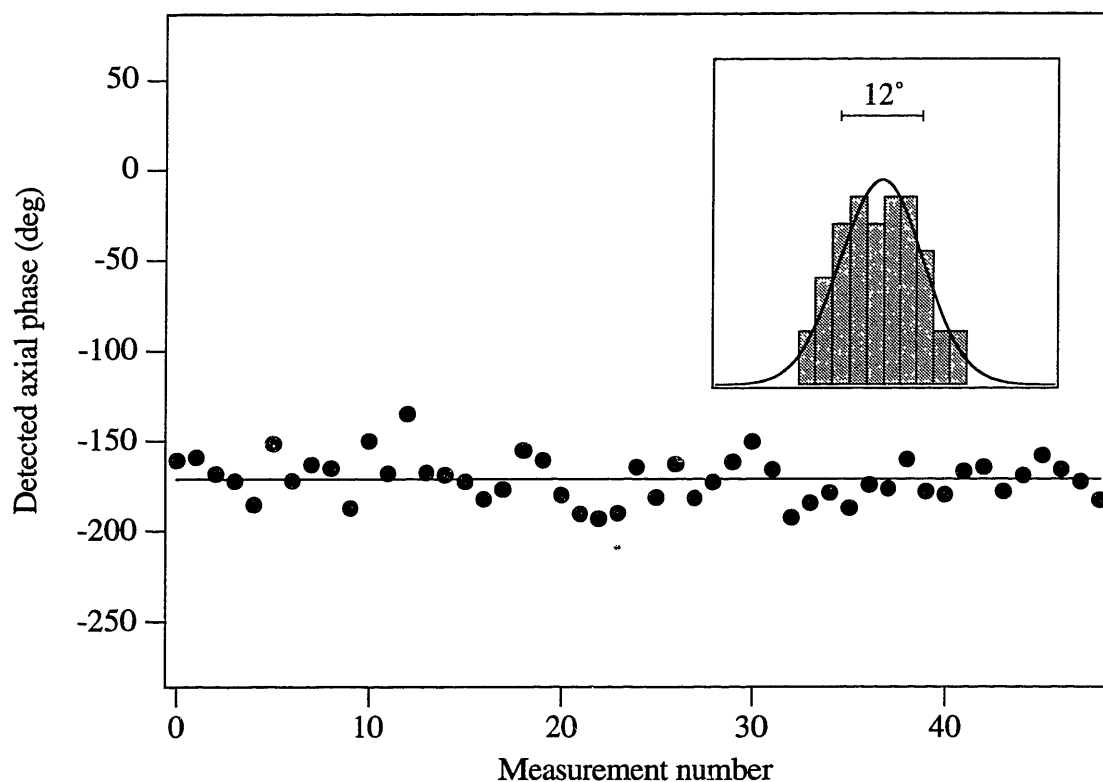
Fig. 2-3 Phase estimation noise for Ne^+ . The axial phase is measured after exciting the cyclotron mode with a fixed phase and applying a \pi -pulse after 100 ms.
