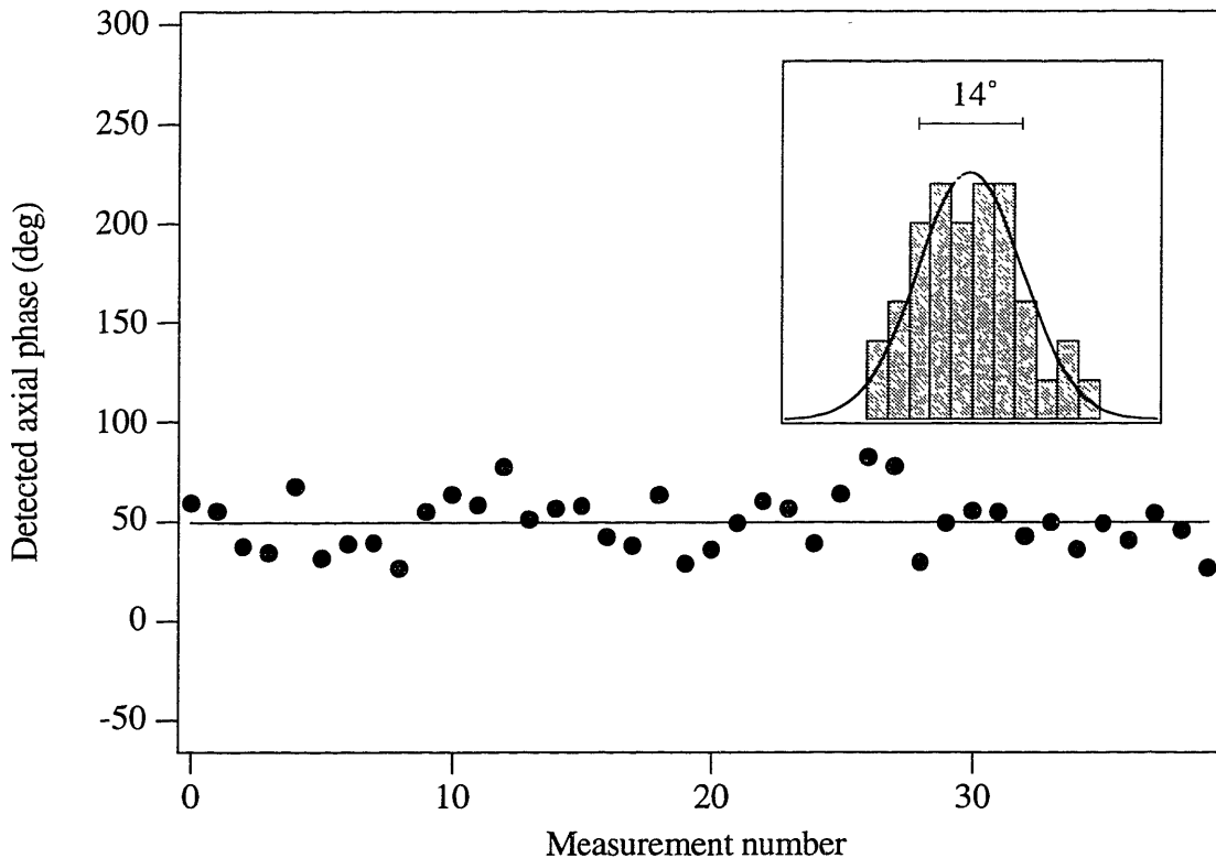
Fig. 4-3 Modified PNP for non-doublets. Each plotted point corresponds to the detected phase in the axial motion of an \text{Ar}^{++} ion after the following experiment. The cyclotron motion was first excited in a non-resonant trap, allowed to evolve for 250 ms, then the trap voltage was changed to make \text{Ar}^{++} resonant, and finally a \pi -pulse was applied after a 2.85 s wait to allow the voltage to stabilize. Some of the phase noise is due to actual magnetic field noise in the 3 seconds of total phase integration. If the correlation with the external magnetometer is removed, the residual phase noise is 11^\circ .
