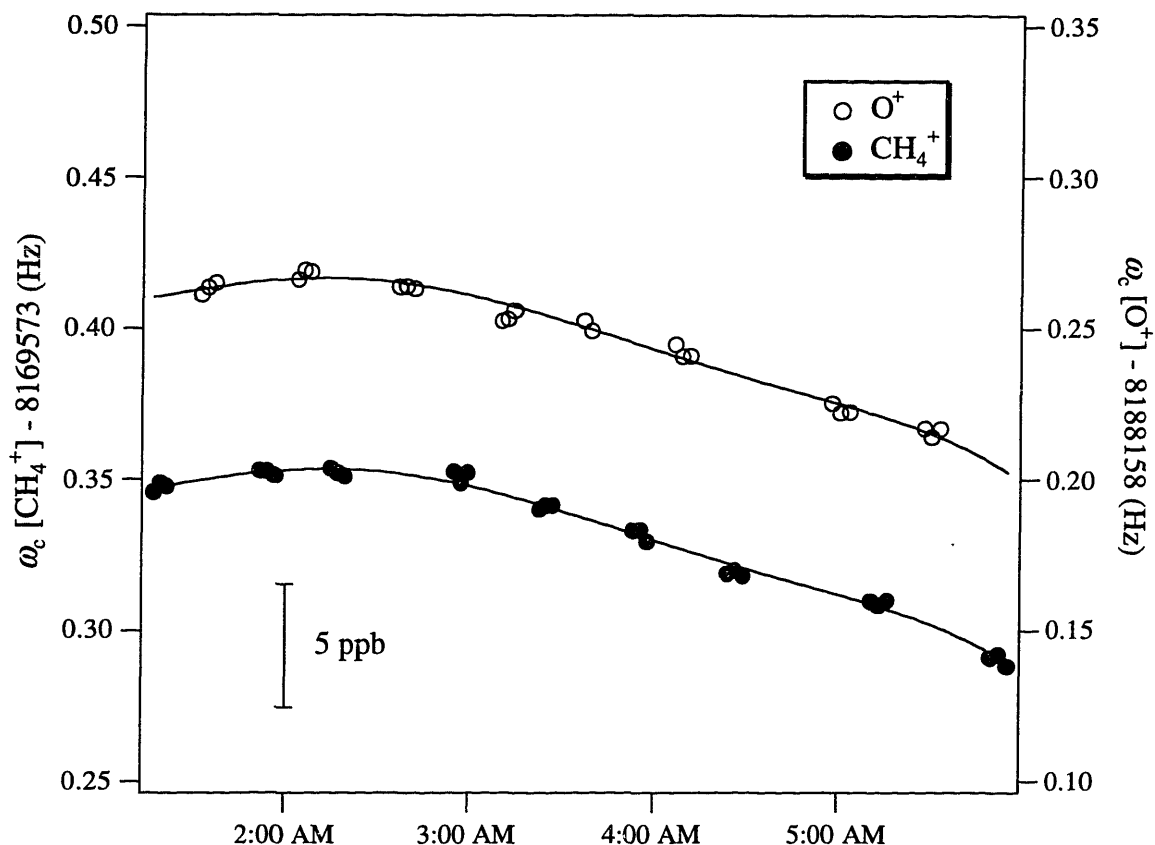
Fig. 3-5 \text{O}^+ vs. \text{CH}_4^+ comparison. The free space cyclotron frequencies for the two ions are plotted as a function of time. The solid lines are a polynomial fit to the magnetic field variation.
