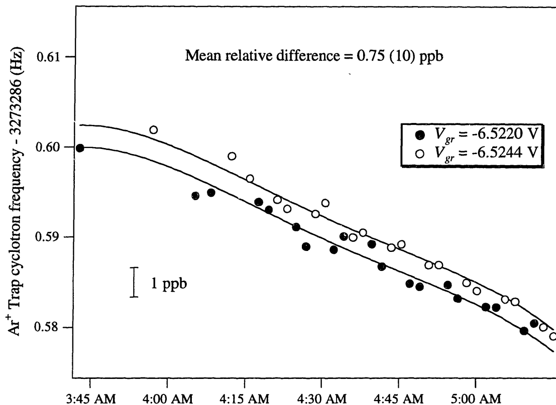
Fig. 3-10 Effect of guard ring voltage on the cyclotron frequency of an Ar + ion. The solid line is a 4th order polynomial fit to the field drift.
