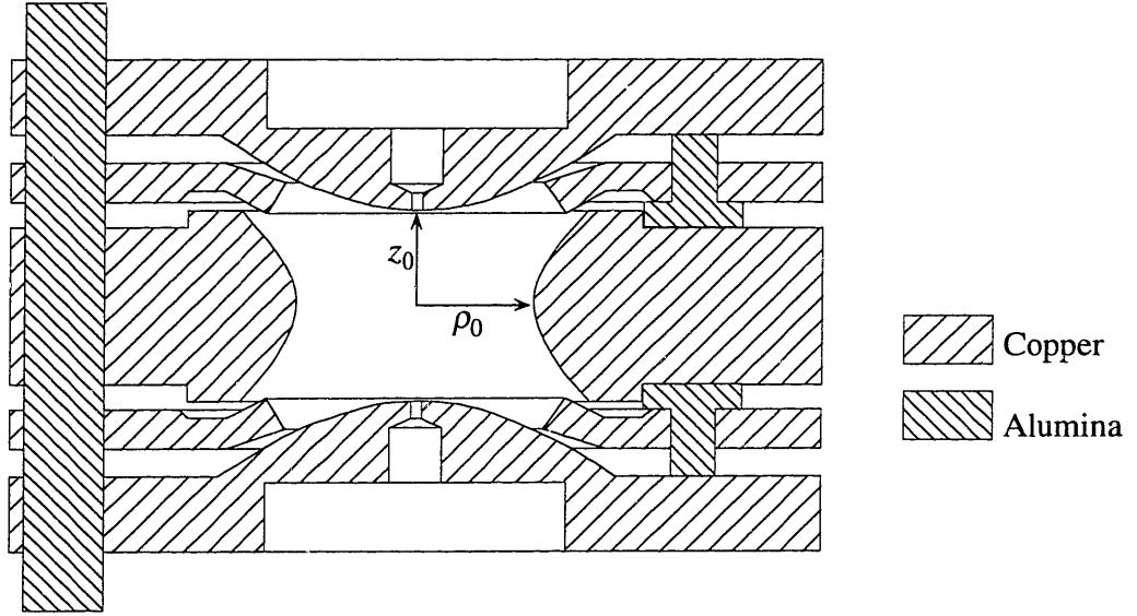
Fig. 1-2 Cross sectional view of an assembled trap. The endcap electrodes follow the equation z^2 - \rho^2/2 = z_0^2 while the ring electrode follows z^2 - \rho^2/2 = \rho_0^2/2 . In our trap, z_0 = 0.600 cm and \rho_0 = 0.696 cm, giving a characteristic size d^2 = 0.301 cm 2 .
