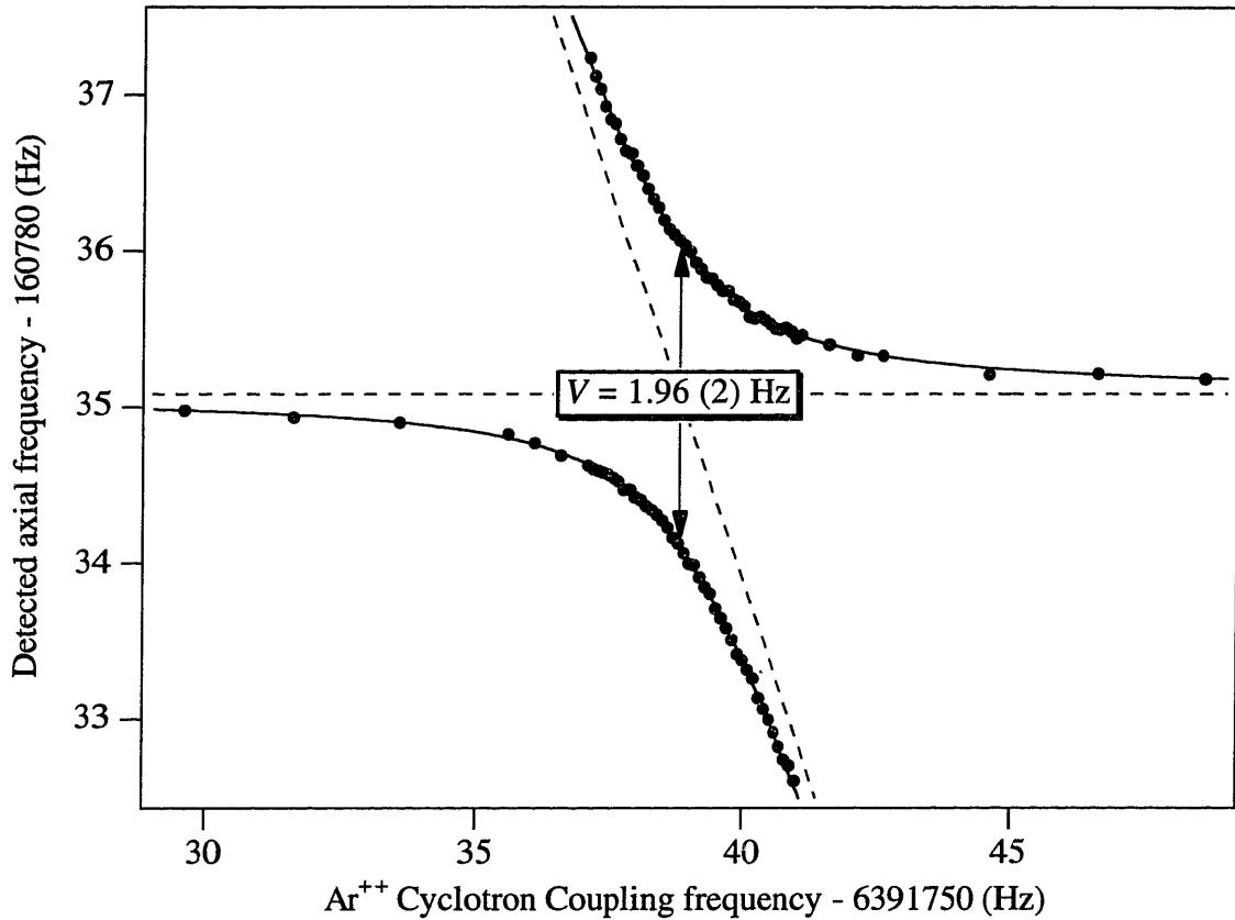
Fig. 3-2 Cyclotron avoided crossing for \text{Ar}^{++} . The frequencies of the two states that appear near the detector are plotted as the coupling frequency is scanned through the resonance. The actual detected signals from which the frequencies were extracted are shown in Fig. 1-3.
