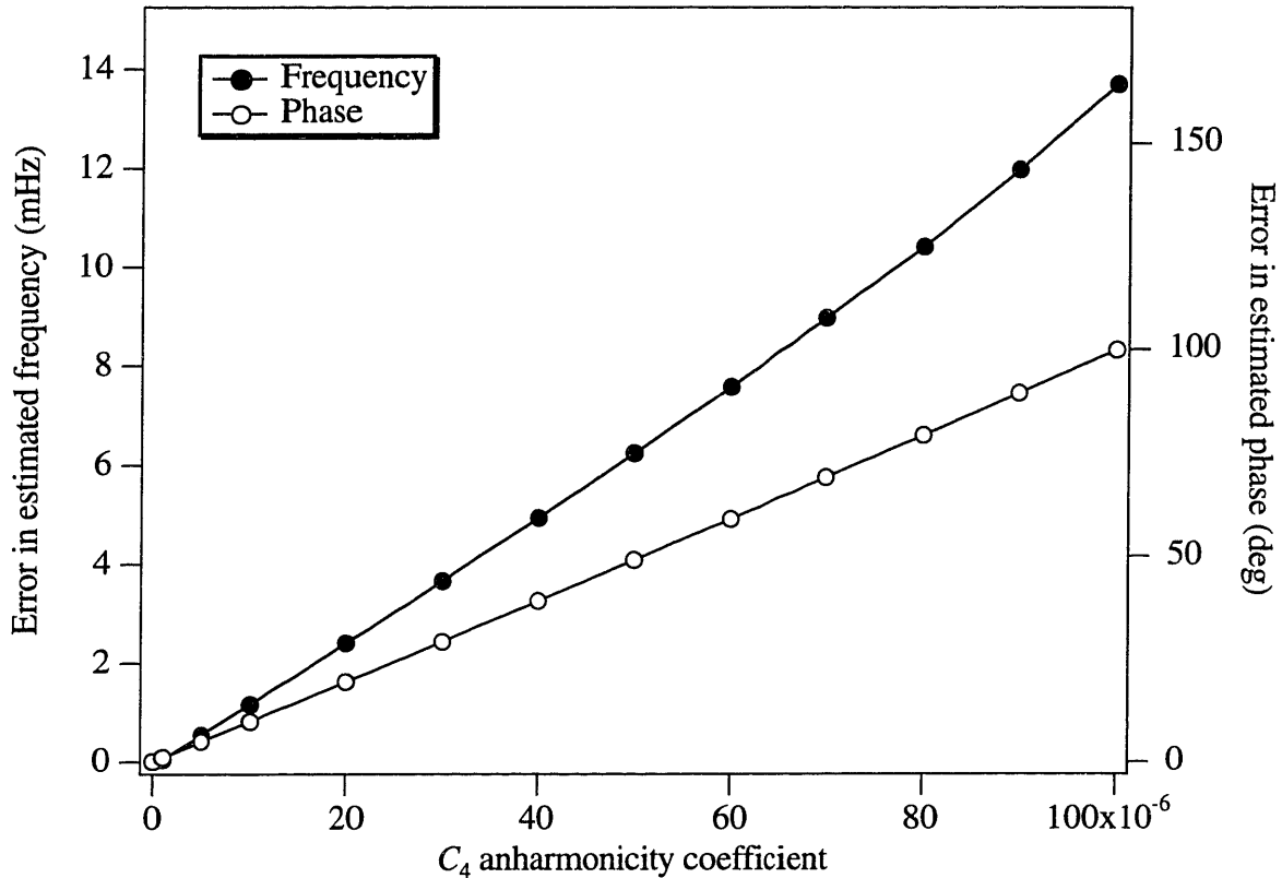
Fig. 2-2 The effect of small anharmonicity on estimated parameters. The errors in the estimated frequency and phase are shown as a function of C_4 (see text). The data consisted of 2048 points sampled at 250 Hz with a damping time of 4 s.
