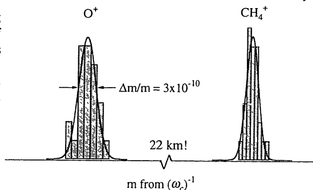
Fig. 1-1. Development of mass spectrometry. This figure shows the chronological improvement in the precision of mass measurements from 1950-1993. In all cases the two peaks shown form a doublet, although the doublet separations are not exactly the same.
