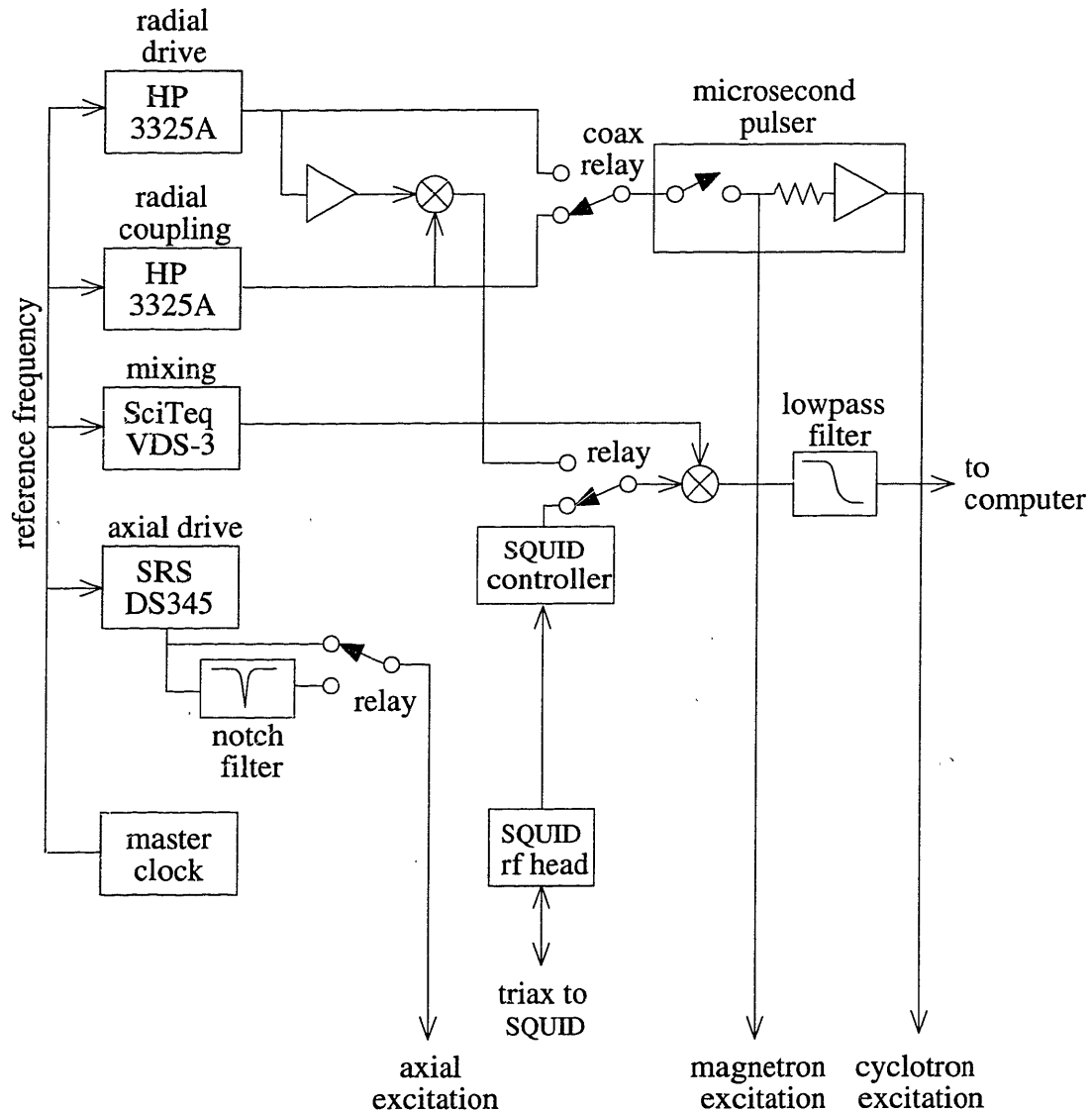
Fig. 1-5 The driving and detecting electronics. The relays are all controlled by the computer, as are all the signal generators except the SciTeq.
