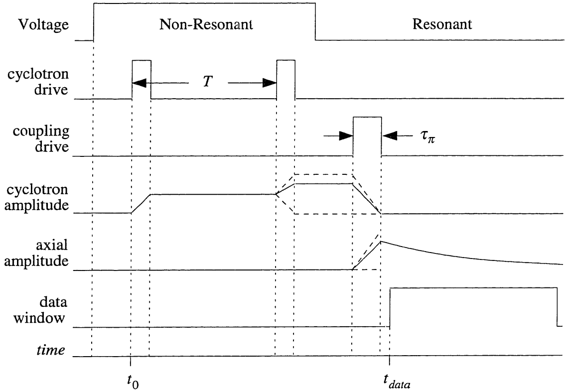
Fig. 4-2 Driving sequence for the SOF measurement (not to scale). The voltage settings are selected for driving (non-resonant) and coupling to the axial (resonant). The cyclotron amplitude depends on the separation time between the pulses T , but is bounded between 0 and 2A . Except for T , the timing of all the other pulses is non-critical.
