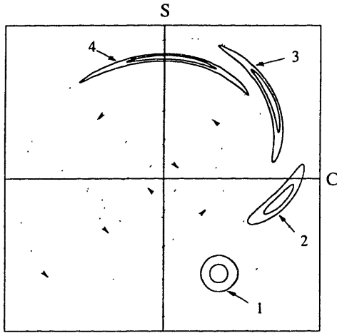
FIG. 1. Amplitude squeezing for an anharmonic oscillator driven at 2\omega_0 for \gamma < 0 . Initial Gaussian contours (1) are transformed along the phase trajectories in the C - S plane (dotted lines) through intermediate states (2) and (3) until amplitude uncertainty is reduced (4). (The \gamma > 0 diagram is obtained by reflecting about either axis.)
