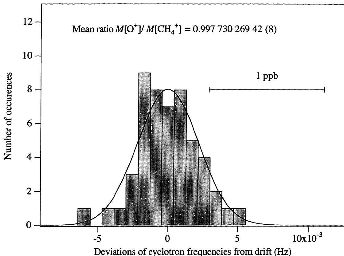
Fig. 3-8 Histogram of frequency deviations around drift. The residuals in the cyclotron frequency of both ions around the drift is accounted for in this histogram.
