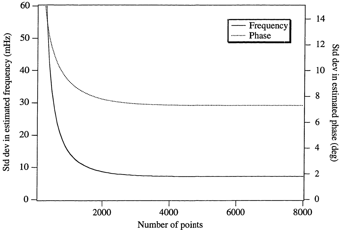
Fig. 2-1 Cramer-Rao bounds for estimation error. The lower bounds on the standard deviation in the estimated frequency and phase are shown as a function of the number of data points, and hence the total sampling time. The damping time was 4 s, the sampling rate was 250 Hz, and the signal to noise was adjusted for our current levels.
