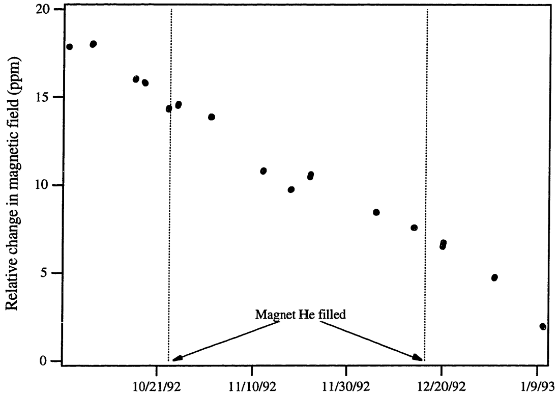
Fig. 2-10 Long term drift in the magnetic field. The magnet liquid He cryostat was filled on the days shown. The DC magnetic field is 8.5285 T.
