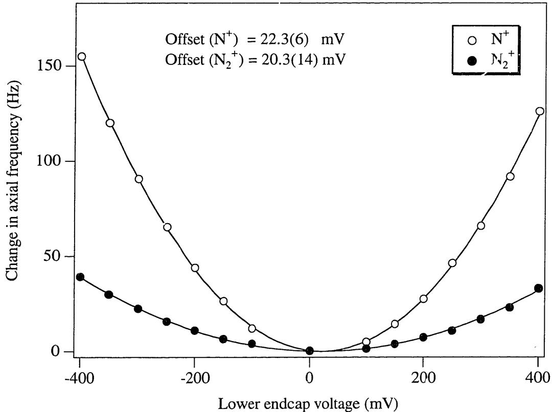
Fig. 4-1 Axial patch effect measurement with N^+ and N_2^+ . The axial frequency shifts quadratically with the applied voltage on the lower endcap. The minimum of the parabola indicates the electrical center of the trap and should lie at 0 applied voltage if there were no patch effect offset.
