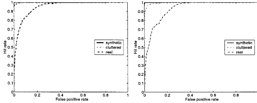
(a) face only features
