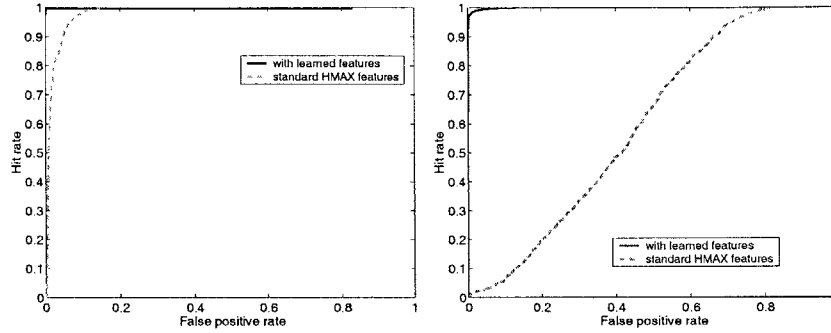
(a) synthetic faces and non-faces (b) cluttered faces and non-faces
