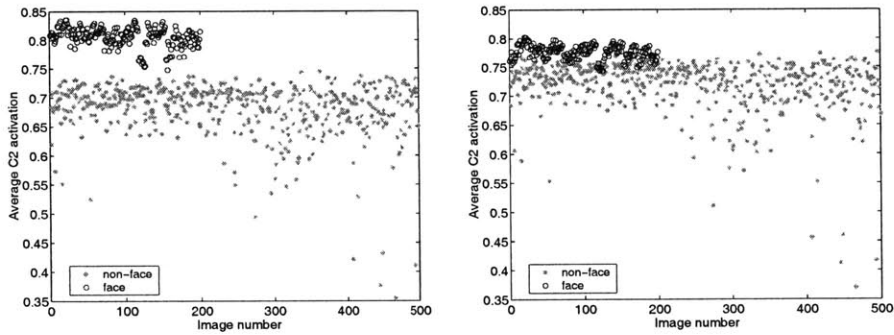
Figure 4-2: Average C2 activation of training sets. Left: using face only features. Right: using mixed features.
