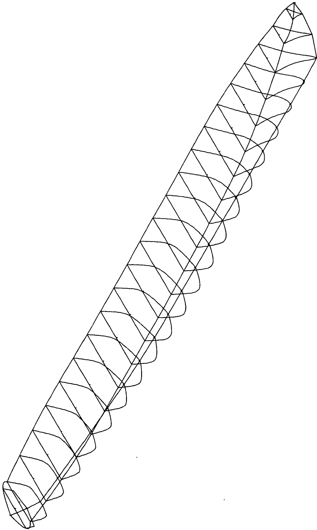
Figure 4-2: SHCP Isometric View of FFG36-61
