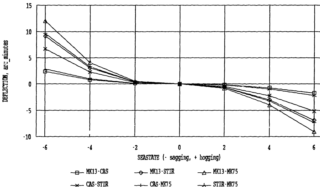
FIG 6-1-PULL LOAD CONDITION, DEFLECTIONS BETWEEN ELEMENTS, REL. TO SEASTATE 0
