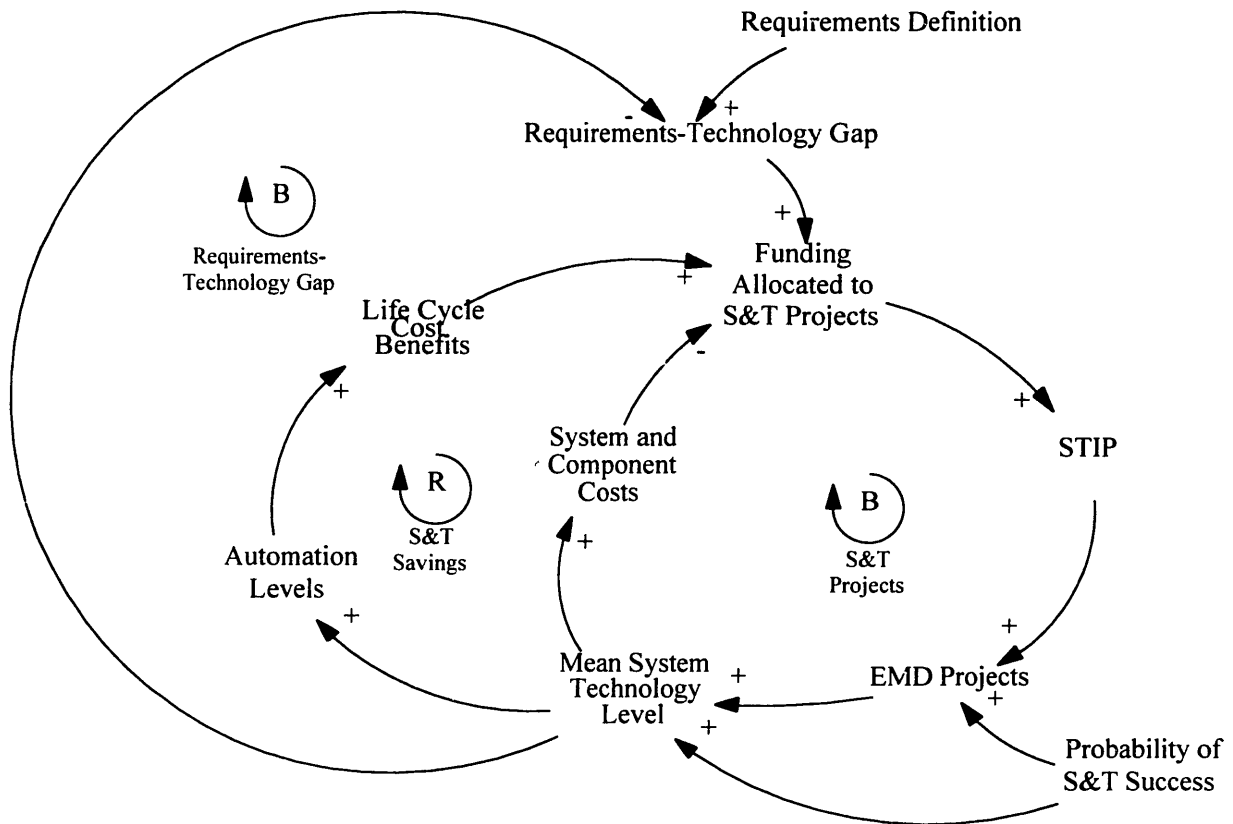
Figure 4: S&T Causal Loop Diagram
