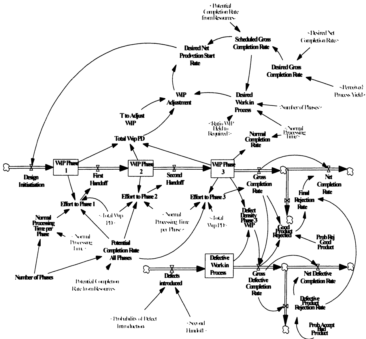
Figure 6: SCIP Model, Production Product Development Segment
