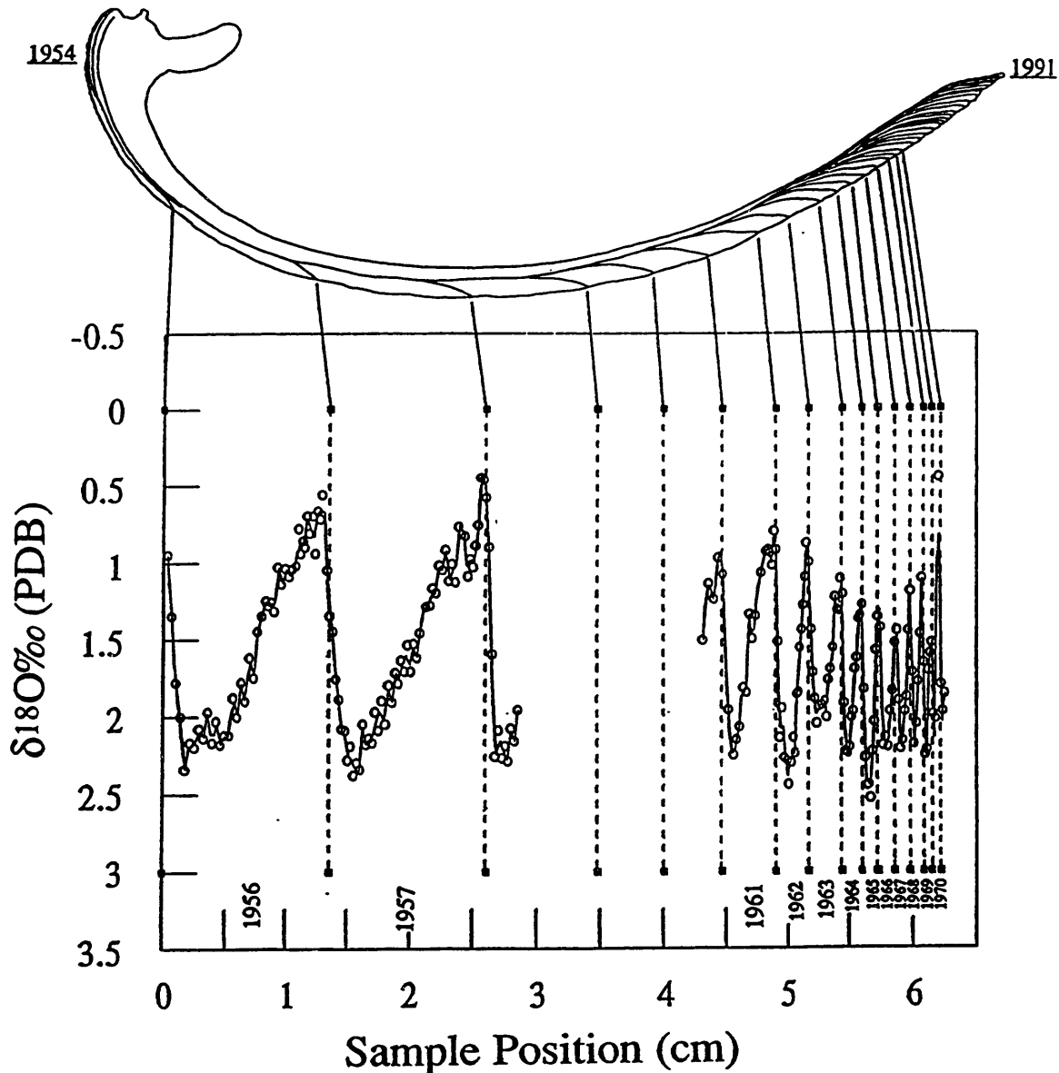
Figure 4. Shell \delta^{18}\text{O} composition versus cumulative sample position. The seasonal \delta^{18}\text{O} signal is in phase with the banding pattern, and the annual "marks" (represented by vertical dashed lines) are deposited at or just after the seasonal \delta^{18}\text{O} minima (or bottom temperature maxima). As shown in the radial cross section through the shell, annual bandwidths decrease with age, reducing sampling resolution (and temporal resolution) in the outermost bands.
