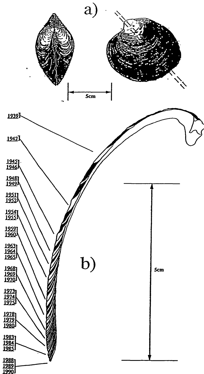
Fig. 3. (a) Two views of a typical 50-year-old A. islandica specimen. One of the valves is radially sliced, along its axis of maximum linear growth. (b) Tracing of a photoclargement of a thin-section obtained from the same 54-year-old Georges Bank A. islandica specimen used in this study. The white areas indicated in the outer shell layer correspond to the annual growth bands analyzed for radiocarbon, while the dark areas correspond to the bands that were not analyzed. Less temporal resolution is achieved in the samples comprised of more recently deposited bands due to a reduction in linear growth rate as the specimen aged.
