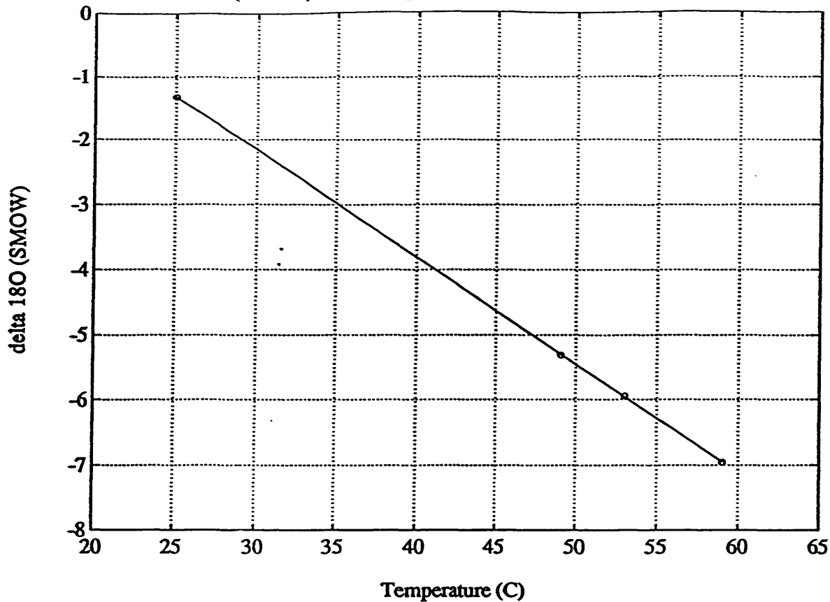
delta 18O (SMOW) of CO2 Equilibrated with Water as F(Temperature C)
