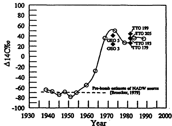
Fig. 7. Estimated Labrador Sea \Delta^{14}\text{C} time history (using equation (6)) compared with mixed layer \Delta^{14}\text{C} measurements from two GJOSECS and four TTO stations in and adjacent to the Labrador Sea (the uppermost two \Delta^{14}\text{C} values from each station were used to calculate a mean for the layer 0-100 m). The prebomb mean of -70.6‰ is lower than the -55‰ previously used to estimate the bomb ^{14}\text{C} inventory for the Labrador Sea [Broecker et al. , 1985], though almost identical to the -70‰ estimated for prebomb NADW source waters [Broecker, 1979]. Seawater \Delta^{14}\text{C} measurements in the Labrador Sea region in the 1970s and 1980s are in general agreement with our estimated \Delta^{14}\text{C} time history. Standard errors for GJOSECS and TTO data are smaller than symbols.
