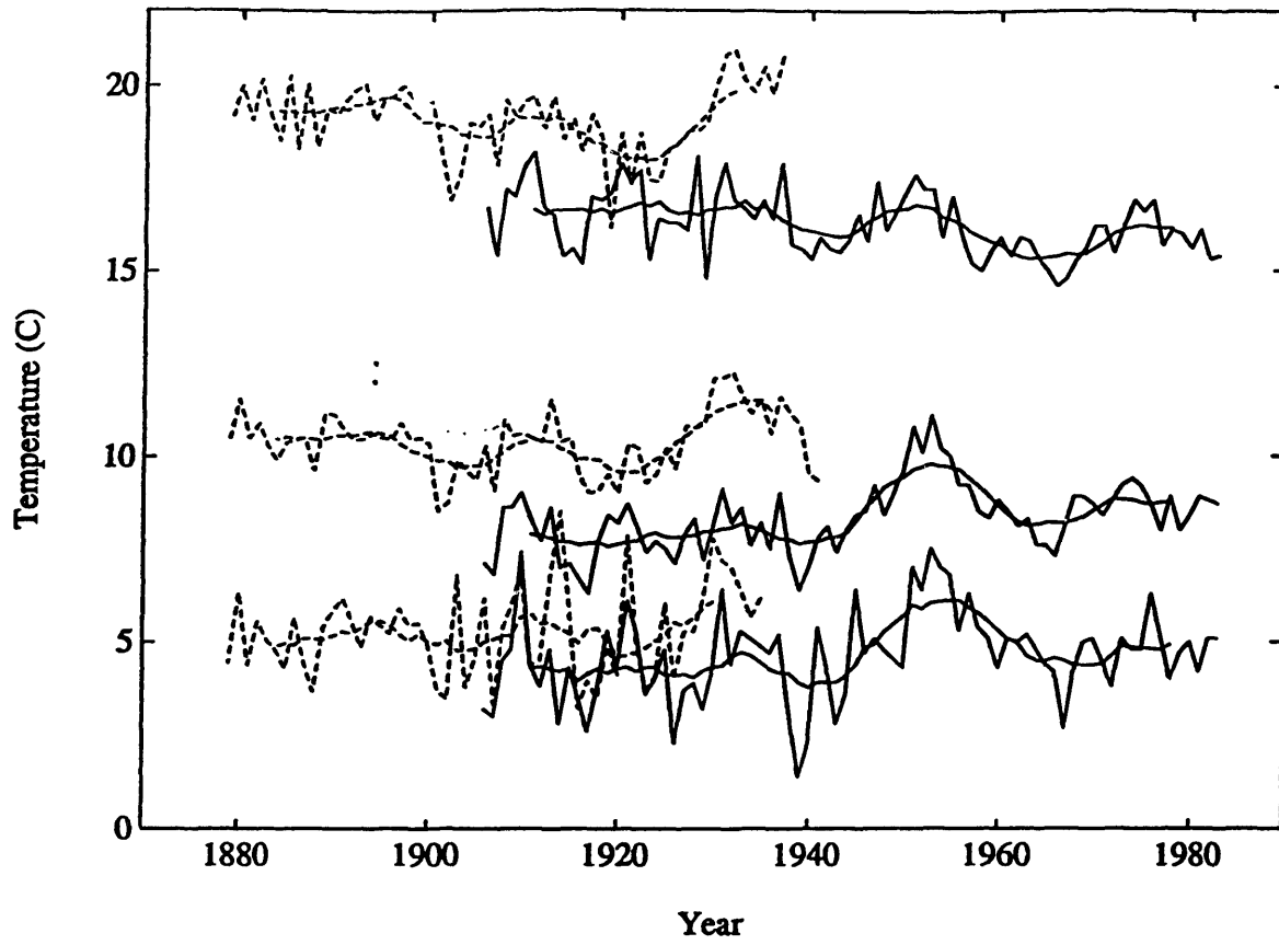
Boothbay & Brenton Reef SST w/ 10-yr running mean
