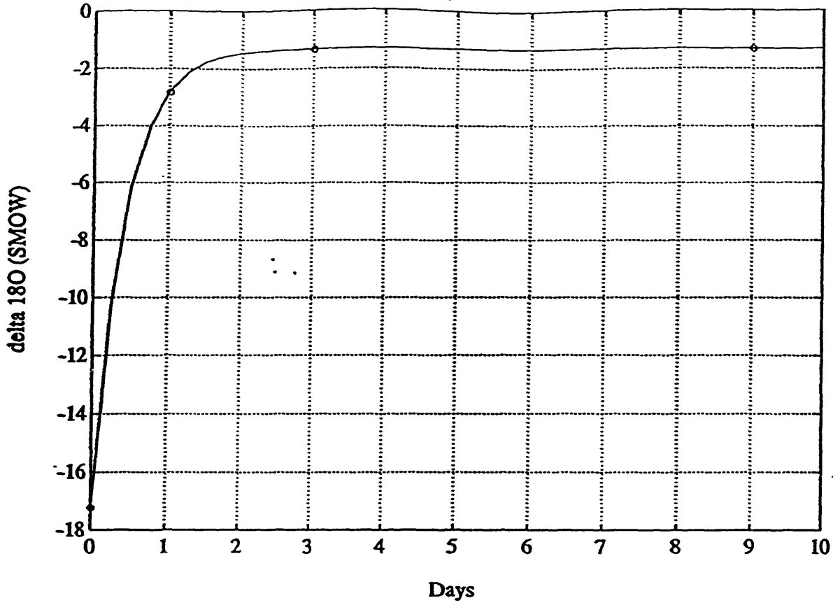
delta 18O (SMOW) of CO 2 Equilibrated with Water as f( time)
