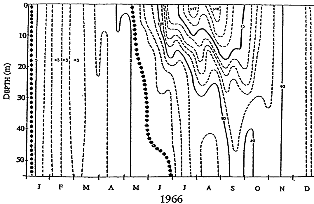
Figure 2. Hydrographs of the seasonal temperature evolution of the water column at the Nantucket Shoals Lightship for the years 1963 and 1966 (adapted from Chase, [1966, 1969b]). The dotted lines are the 6°C isotherms. Bottom temperatures are at or above 6°C from about May to December and below 6°C from January to April. Note that both years show a similar evolution and range of surface temperatures, while the bottom experiences a much colder year in 1966 than in 1963, with maximum bottom temperatures 4°C lower in 1966.
