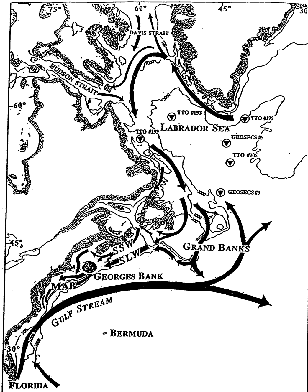
Fig. 2. Schematic of the major surface flow patterns of the northwestern Atlantic Ocean [after Chapman et al. , 1986] is shown along with the positions of GEOSECS and TTO stations in and peripheral to the Labrador Sea. The A. islandica collection site on Georges Bank is marked with a clam-shaped symbol. Chapman and Beardsley [1989] have described the shelf waters on the southern flank of Georges Bank as 75% Scotian Shelf Water (SSW) and 25% Slope Water (SLW), with both components originating in the Labrador Sea.
