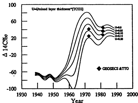
Fig. 8. Sensitivity of the Labrador Sea estimate to uptake rate U . The model shows the sensitivity of the estimated \Delta^{14}\text{C} value during the bomb period when the atmosphere-ocean \Delta^{14}\text{C} difference was large. U here is constrained by the GEOSECS and TTO \Delta^{14}\text{C} measurements. Higher uptake rates improve fit with GEOSECS data but worsen fit with TTO data. The prebomb estimate is much less sensitive to U because of the smaller air-sea \Delta^{14}\text{C} difference, but higher rates result in unrealistic \Delta^{14}\text{C} depletions in the Labrador Sea during the peak of the atmospheric bomb signal in the early 1960s.
