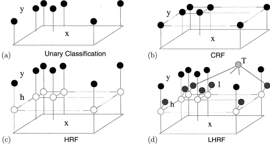
Figure 5-2: Graphical models for different discriminative models of images. The image x and the shaded vertices are observed during training time. The parts h , denoted by unfilled circles, are not observed and are learnt during the training. In the LHRF model, the node corresponding to T is connected to all the locations l_i , depicted using thick dotted lines.
