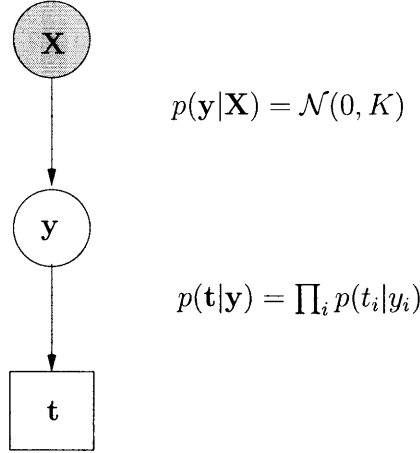
Figure 2-1: Graphical model for Gaussian process classification. Note that, \mathbf{X} = \{\mathbf{X}_L, \mathbf{X}_U\} and is observed for both training and test data points. Also \mathbf{t} = \{\mathbf{t}_L, \mathbf{t}_U\} ; however, only \mathbf{t}_L corresponding to the labeled data points are observed.
