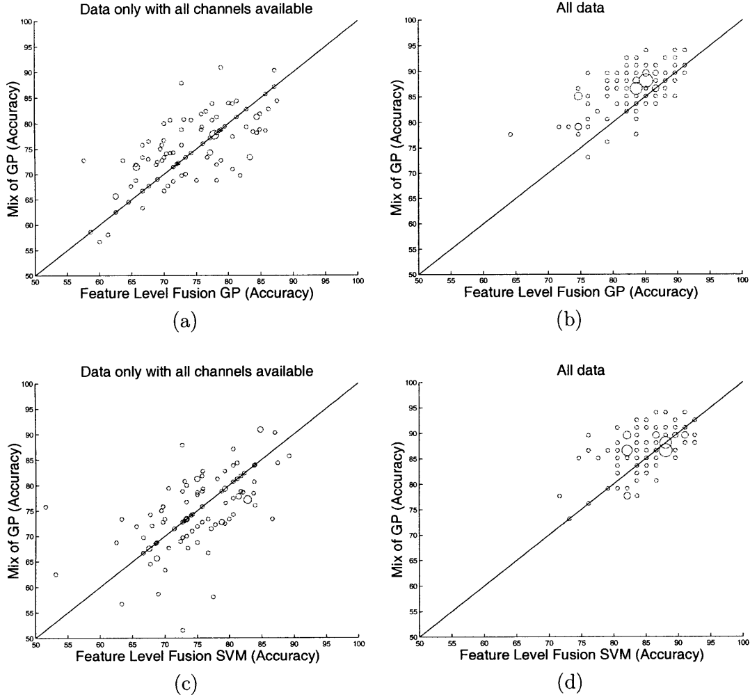
Figure 3-7: Plots comparing accuracy of Mixture of GP with GP (a)-(b) and SVM (c)-(d) where the latter methods use feature fusion. In (a) and (c) only the subset of data where all modes are intact is used. In (b) and (d) all the data is used, as described in the text. There are 100 points on each graph and each point is (accuracy SVM/GP, accuracy Mixture of GP) and corresponds to one test run. Circle width is proportional to the number of points having that coordinate. Points above the diagonal indicate where Mixture of GP was more accurate. While Mixture of GP is better (a) or comparable (c) on average when all the modes are intact, it is particularly better when there are noisy and missing channels (b) and (d).
