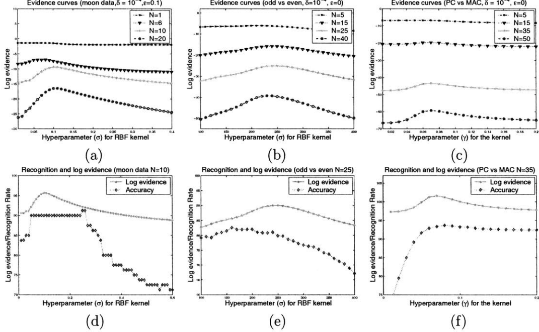
Figure 4-2: Evidence curves showing similar properties across different datasets (half-moon, odd vs even and PC vs MAC). The top row figures (a), (b) and (c) show the evidence curves for different amounts of labeled data per class. The bottom row figures (d), (e) and (f) show the recognition accuracy on unlabeled points and the log evidence, illustrating the correlation between the recognition performance and the evidence.
